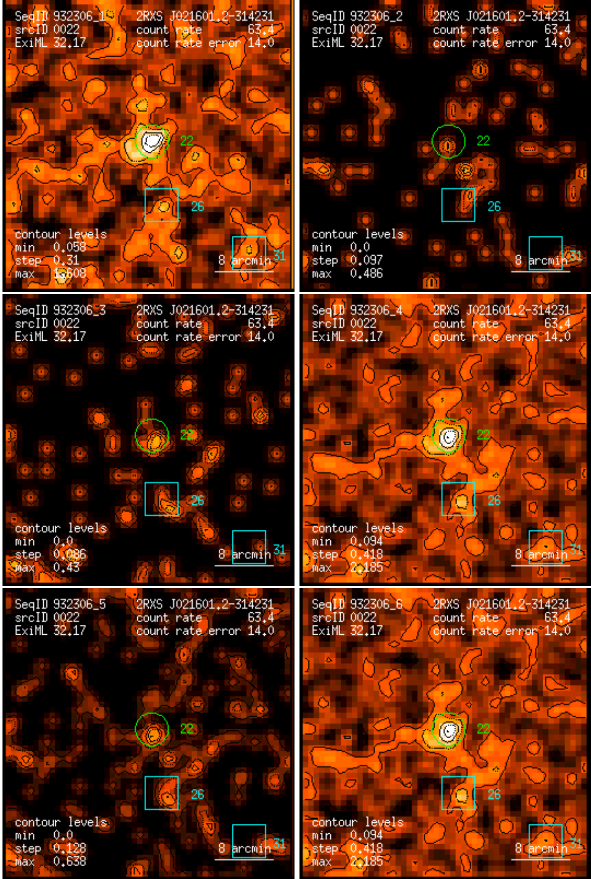
Figure 22: RASS 932306: detection 0022: band rate images, Gaussian filter: (1) PSPC channels 11 – 41, (2) 52 – 90, (3) 91 – 201, (4) 11 – 235, (5) 52 – 201, (6) 11 – 201. Broad band rates in counts/ks. Band rate contour levels in counts/ks/arcmin 2 .
