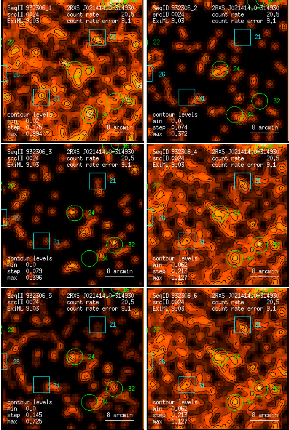
Figure 24: RASS 932306: detection 0024: band rate images, Gaussian filter: (1) PSPC channels 11 – 41, (2) 52 – 90, (3) 91 – 201, (4) 11 – 235, (5) 52 – 201, (6) 11 – 201. Broad band rates in counts/ks. Band rate contour levels in counts/ks/arcmin 2 .
