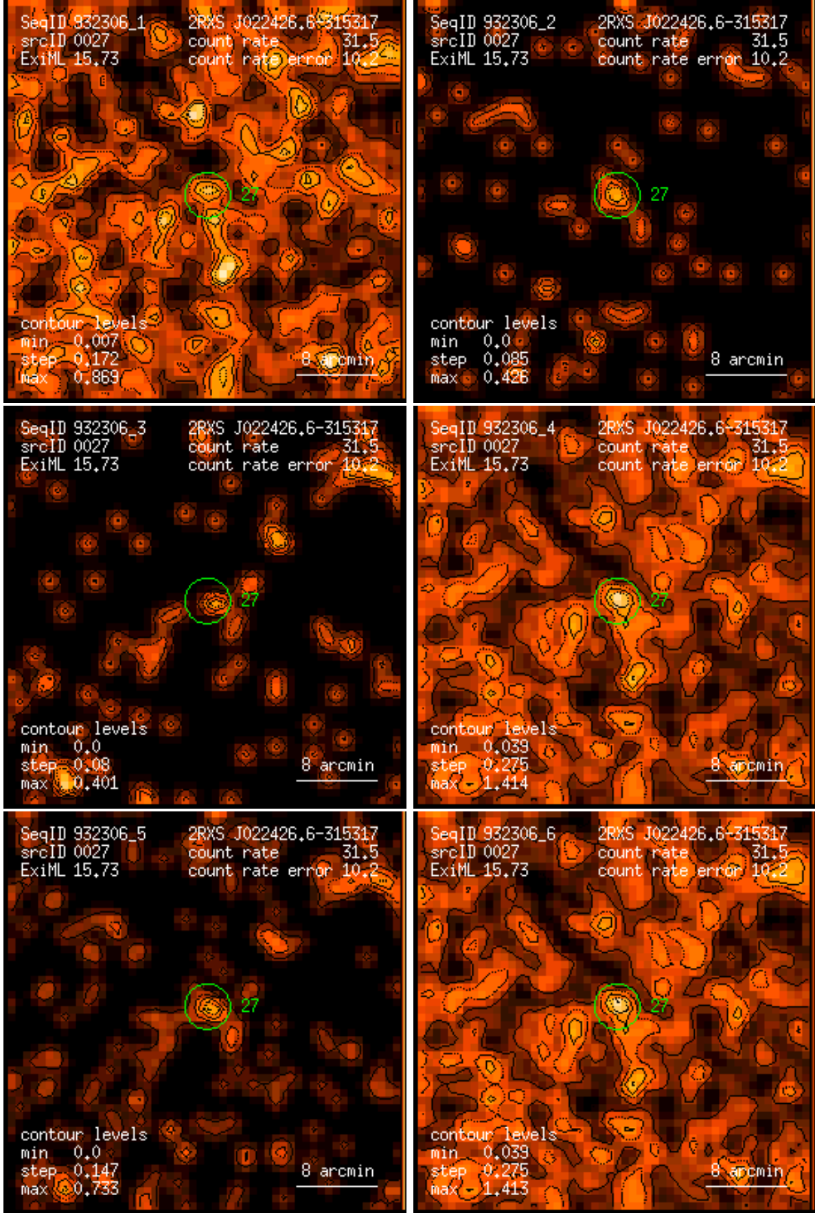
Figure 27: RASS 932306: detection 0027: band rate images, Gaussian filter: (1) PSPC channels 11 – 41, (2) 52 – 90, (3) 91 – 201, (4) 11 – 235, (5) 52 – 201, (6) 11 – 201. Broad band rates in counts/ks. Band rate contour levels in counts/ks/arcmin 2 .
