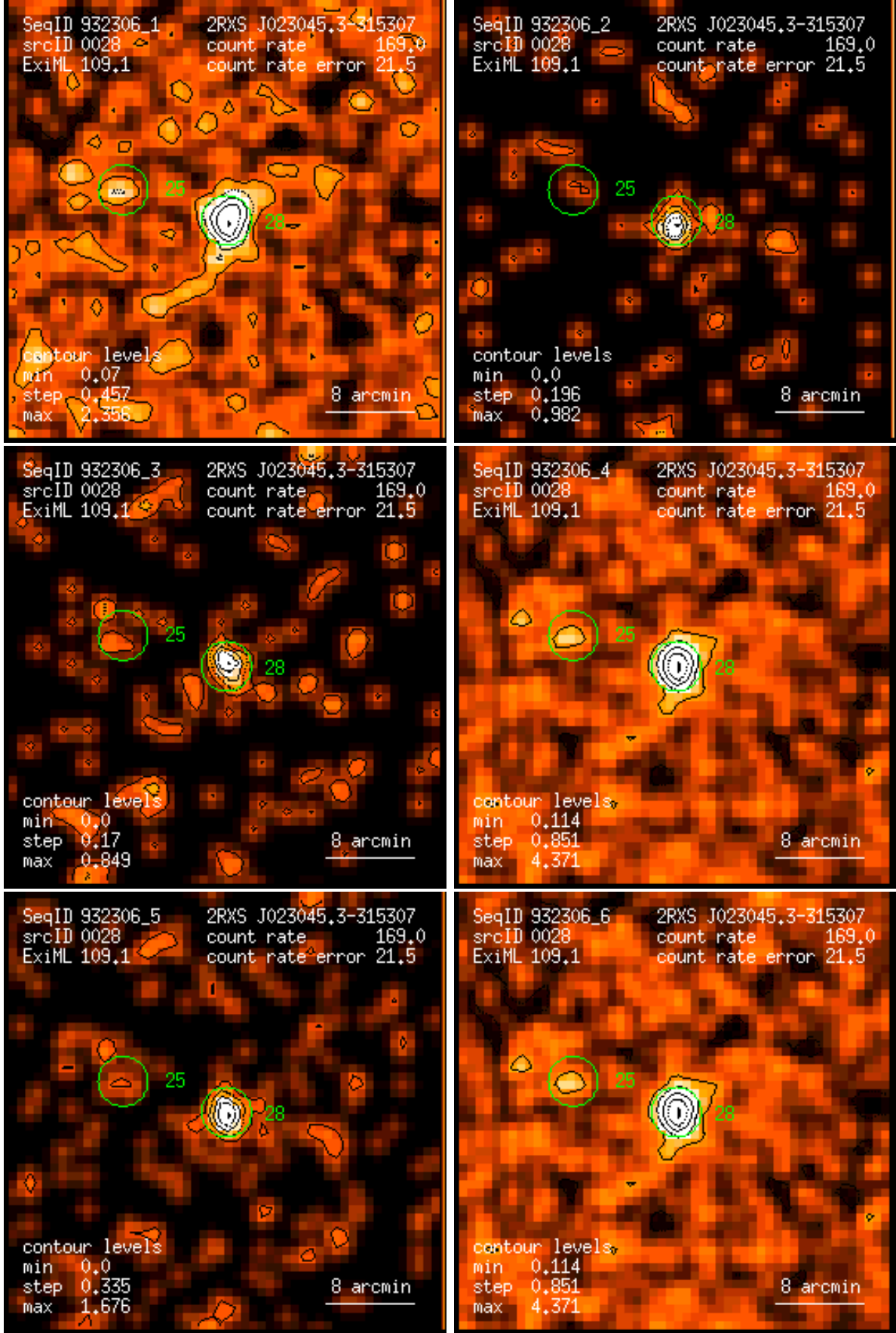
Figure 28: RASS 932306: detection 0028: band rate images, Gaussian filter: (1) PSPC channels 11 – 41, (2) 52 – 90, (3) 91 – 201, (4) 11 – 235, (5) 52 – 201, (6) 11 – 201. Broad band rates in counts/ks. Band rate contour levels in counts/ks/arcmin 2 .
