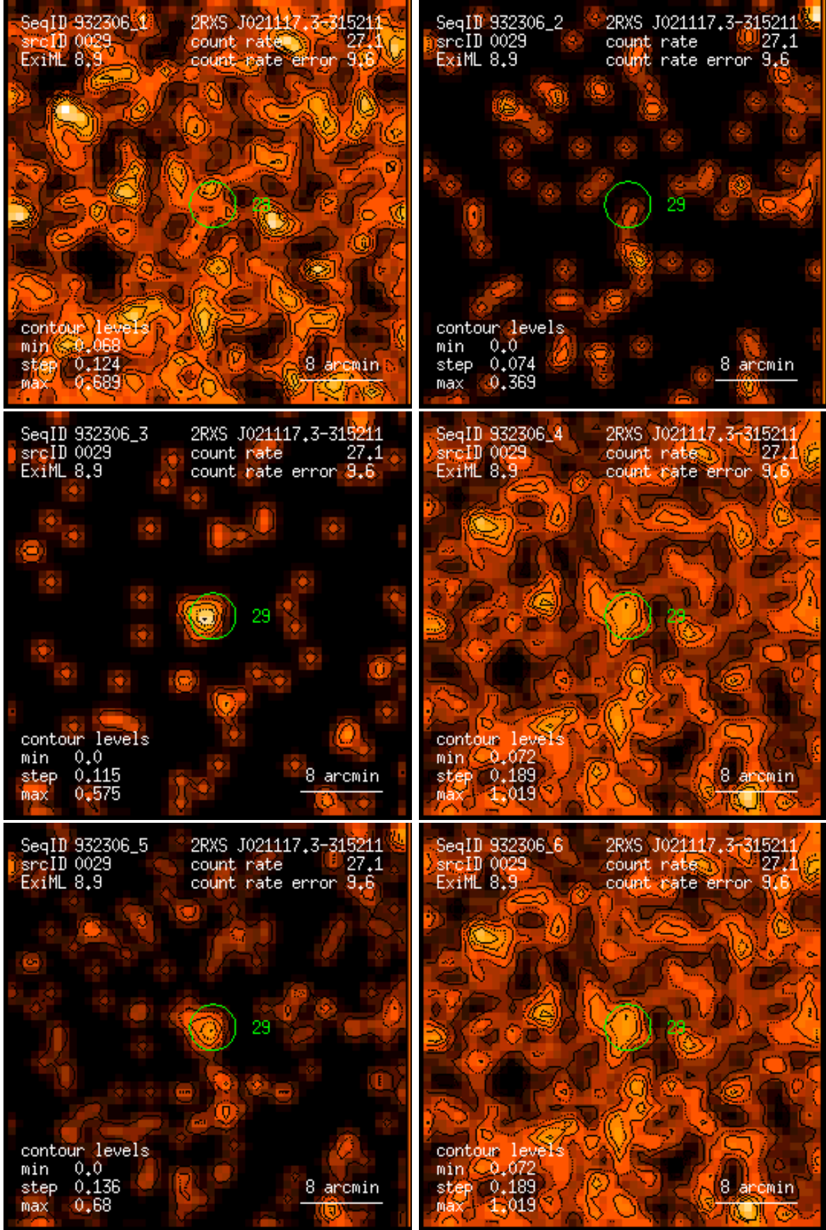
Figure 29: RASS 932306: detection 0029: band rate images, Gaussian filter: (1) PSPC channels 11 – 41, (2) 52 – 90, (3) 91 – 201, (4) 11 – 235, (5) 52 – 201, (6) 11 – 201. Broad band rates in counts/ks. Band rate contour levels in counts/ks/arcmin 2 .
