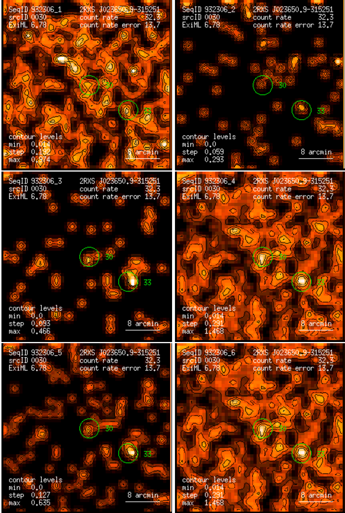
Figure 30: RASS 932306: detection 0030: band rate images, Gaussian filter: (1) PSPC channels 11 – 41, (2) 52 – 90, (3) 91 – 201, (4) 11 – 235, (5) 52 – 201, (6) 11 – 201. Broad band rates in counts/ks. Band rate contour levels in counts/ks/arcmin 2 .
