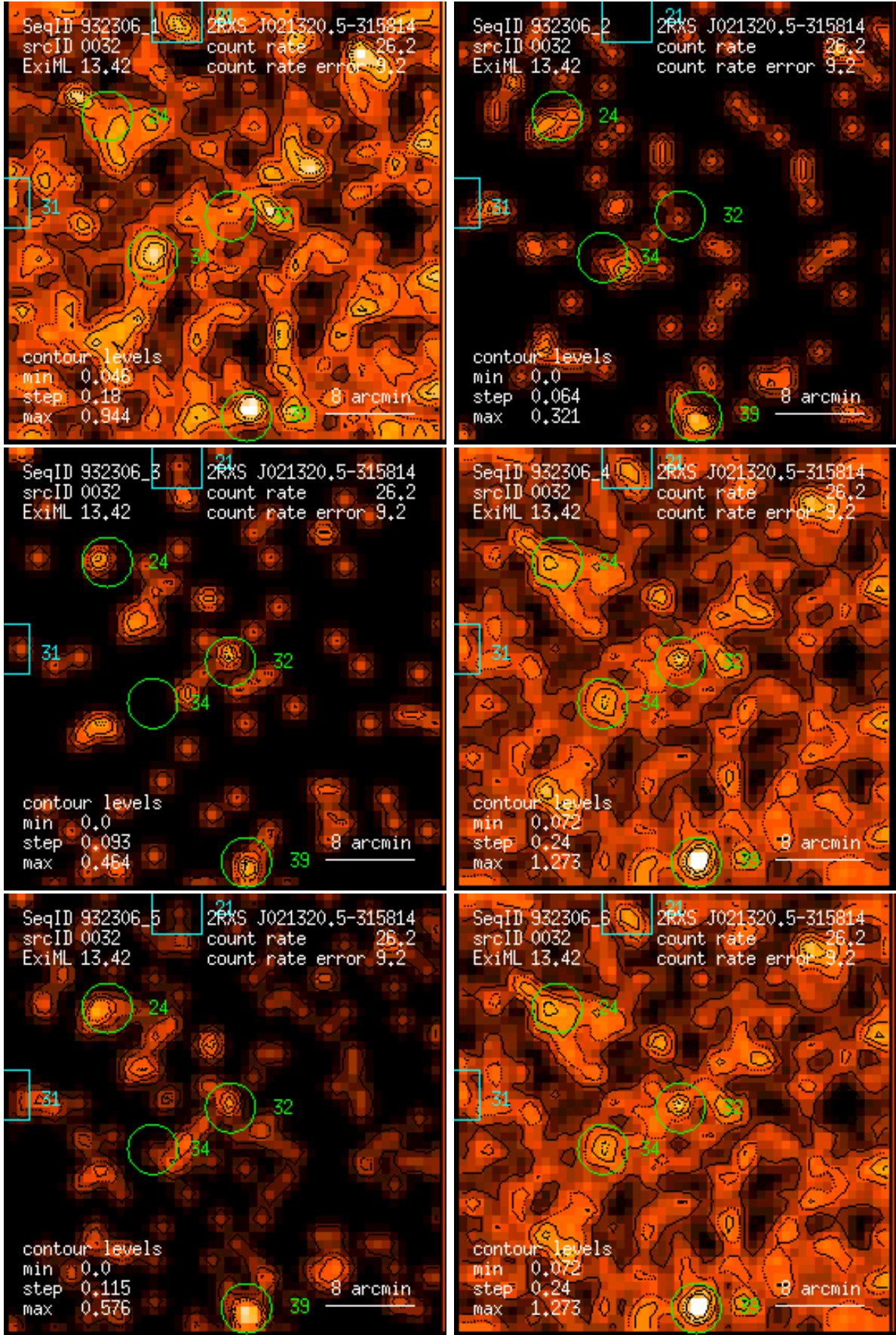
Figure 32: RASS 932306: detection 0032: band rate images, Gaussian filter: (1) PSPC channels 11 – 41, (2) 52 – 90, (3) 91 – 201, (4) 11 – 235, (5) 52 – 201, (6) 11 – 201. Broad band rates in counts/ks. Band rate contour levels in counts/ks/arcmin 2 .
