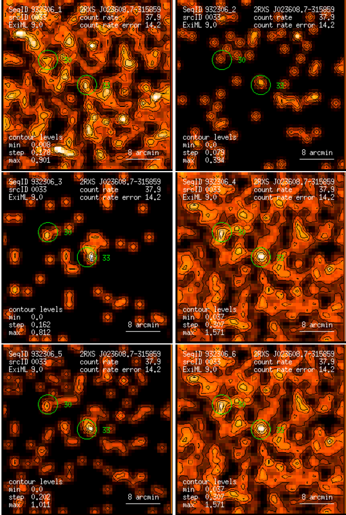
Figure 33: RASS 932306: detection 0033: band rate images, Gaussian filter: (1) PSPC channels 11 – 41, (2) 52 – 90, (3) 91 – 201, (4) 11 – 235, (5) 52 – 201, (6) 11 – 201. Broad band rates in counts/ks. Band rate contour levels in counts/ks/arcmin 2 .
