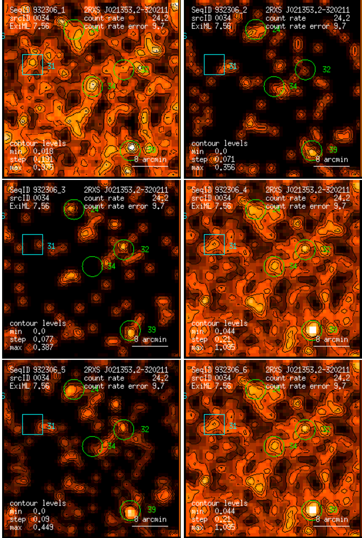
Figure 34: RASS 932306: detection 0034: band rate images, Gaussian filter: (1) PSPC channels 11 – 41, (2) 52 – 90, (3) 91 – 201, (4) 11 – 235, (5) 52 – 201, (6) 11 – 201. Broad band rates in counts/ks. Band rate contour levels in counts/ks/arcmin 2 .
