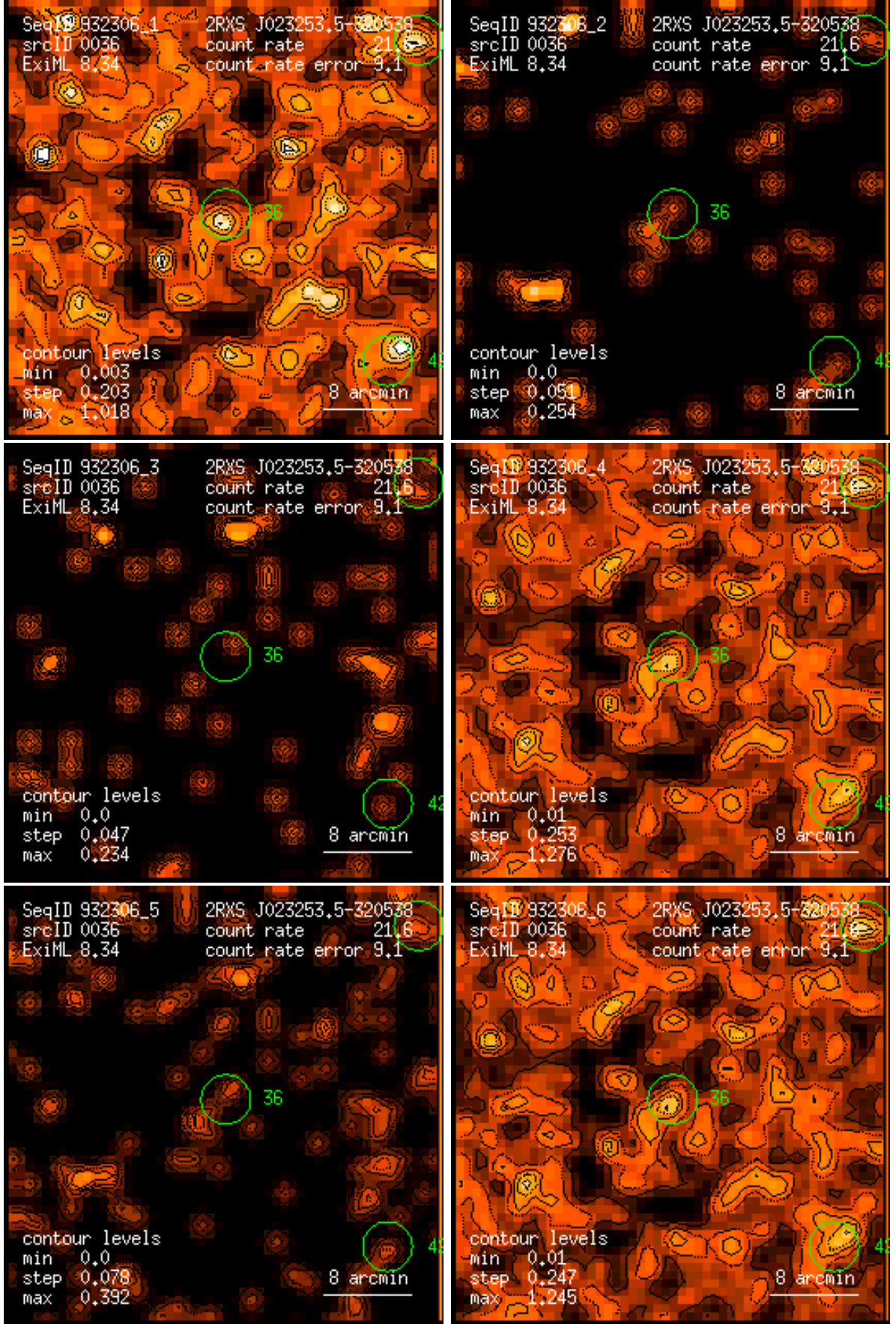
Figure 36: RASS 932306: detection 0036: band rate images, Gaussian filter: (1) PSPC channels 11 – 41, (2) 52 – 90, (3) 91 – 201, (4) 11 – 235, (5) 52 – 201, (6) 11 – 201. Broad band rates in counts/ks. Band rate contour levels in counts/ks/arcmin 2 .
