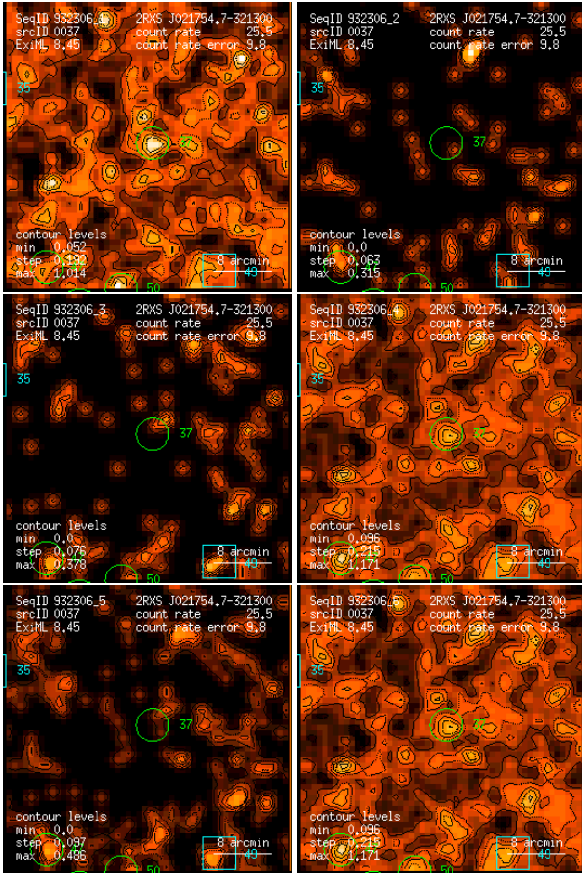
Figure 37: RASS 932306: detection 0037: band rate images, Gaussian filter: (1) PSPC channels 11 – 41, (2) 52 – 90, (3) 91 – 201, (4) 11 – 235, (5) 52 – 201, (6) 11 – 201. Broad band rates in counts/ks. Band rate contour levels in counts/ks/arcmin 2 .
