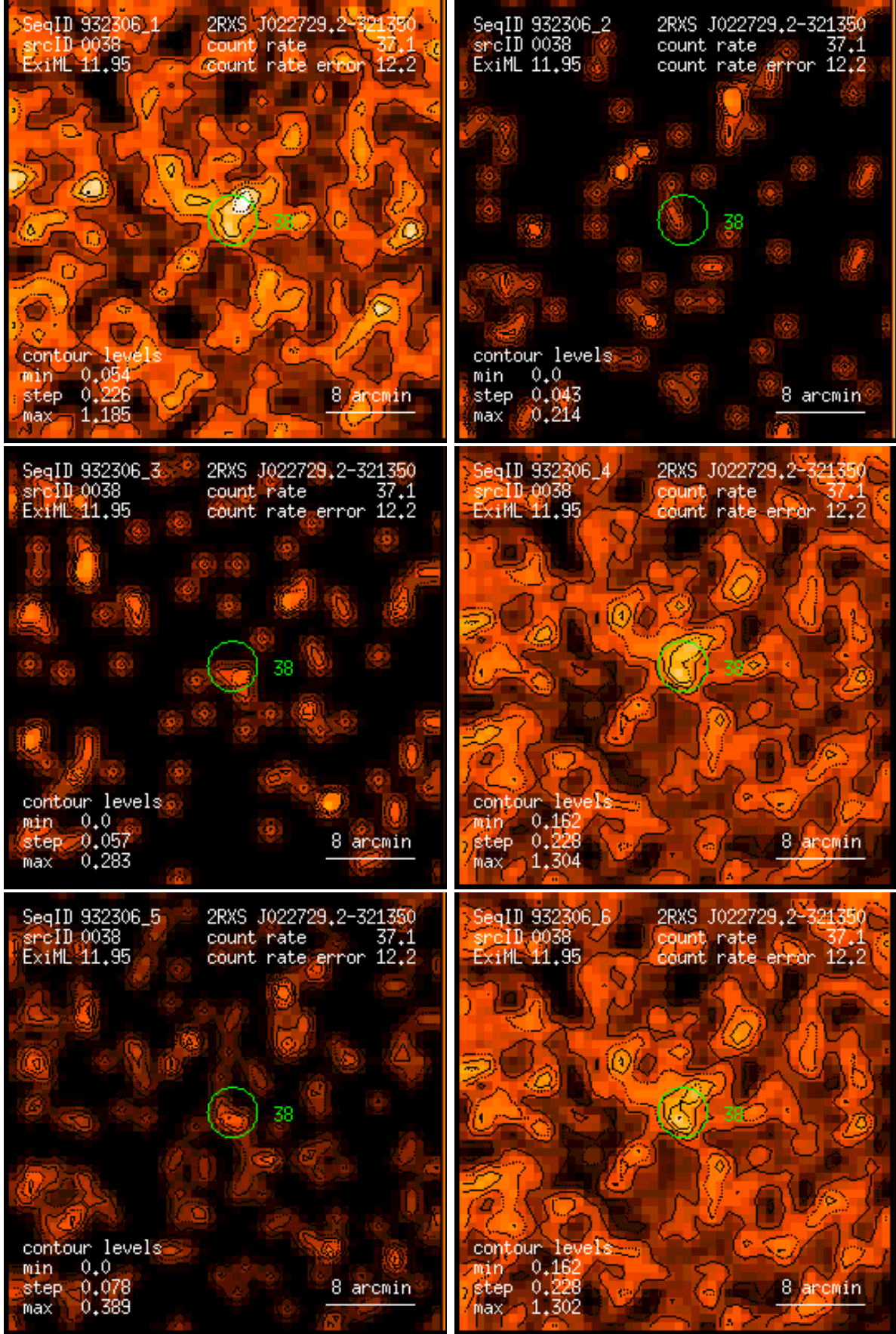
Figure 38: RASS 932306: detection 0038: band rate images, Gaussian filter: (1) PSPC channels 11 – 41, (2) 52 – 90, (3) 91 – 201, (4) 11 – 235, (5) 52 – 201, (6) 11 – 201. Broad band rates in counts/ks. Band rate contour levels in counts/ks/arcmin 2 .
