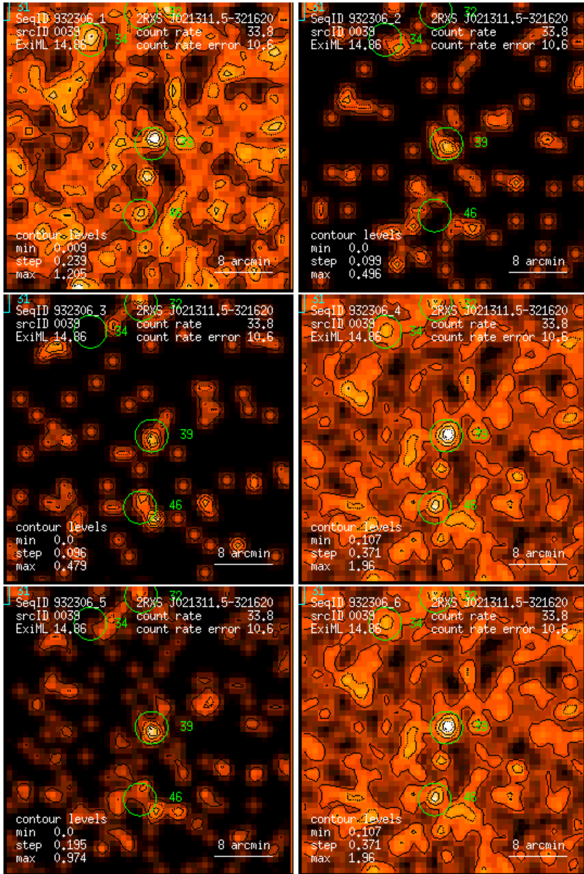
Figure 39: RASS 932306: detection 0039: band rate images, Gaussian filter: (1) PSPC channels 11 – 41, (2) 52 – 90, (3) 91 – 201, (4) 11 – 235, (5) 52 – 201, (6) 11 – 201. Broad band rates in counts/ks. Band rate contour levels in counts/ks/arcmin 2 .
