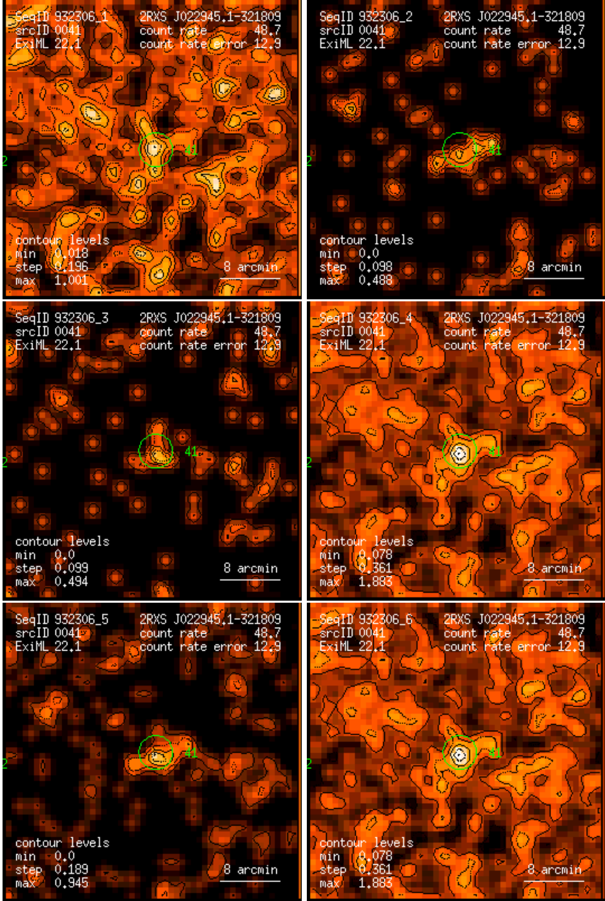
Figure 41: RASS 932306: detection 0041: band rate images, Gaussian filter: (1) PSPC channels 11 – 41, (2) 52 – 90, (3) 91 – 201, (4) 11 – 235, (5) 52 – 201, (6) 11 – 201. Broad band rates in counts/ks. Band rate contour levels in counts/ks/arcmin 2 .
