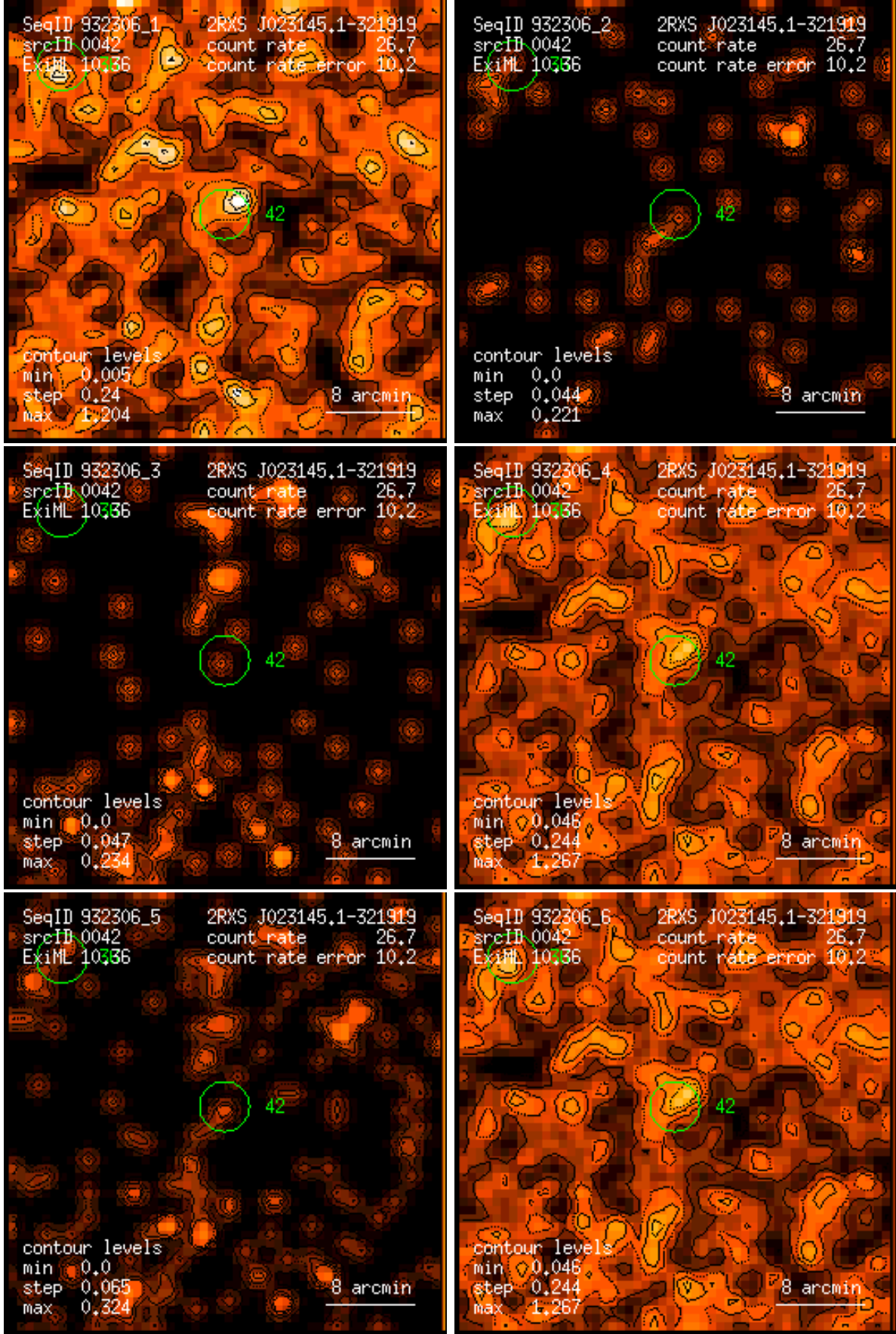
Figure 42: RASS 932306: detection 0042: band rate images, Gaussian filter: (1) PSPC channels 11 – 41, (2) 52 – 90, (3) 91 – 201, (4) 11 – 235, (5) 52 – 201, (6) 11 – 201. Broad band rates in counts/ks. Band rate contour levels in counts/ks/arcmin 2 .
