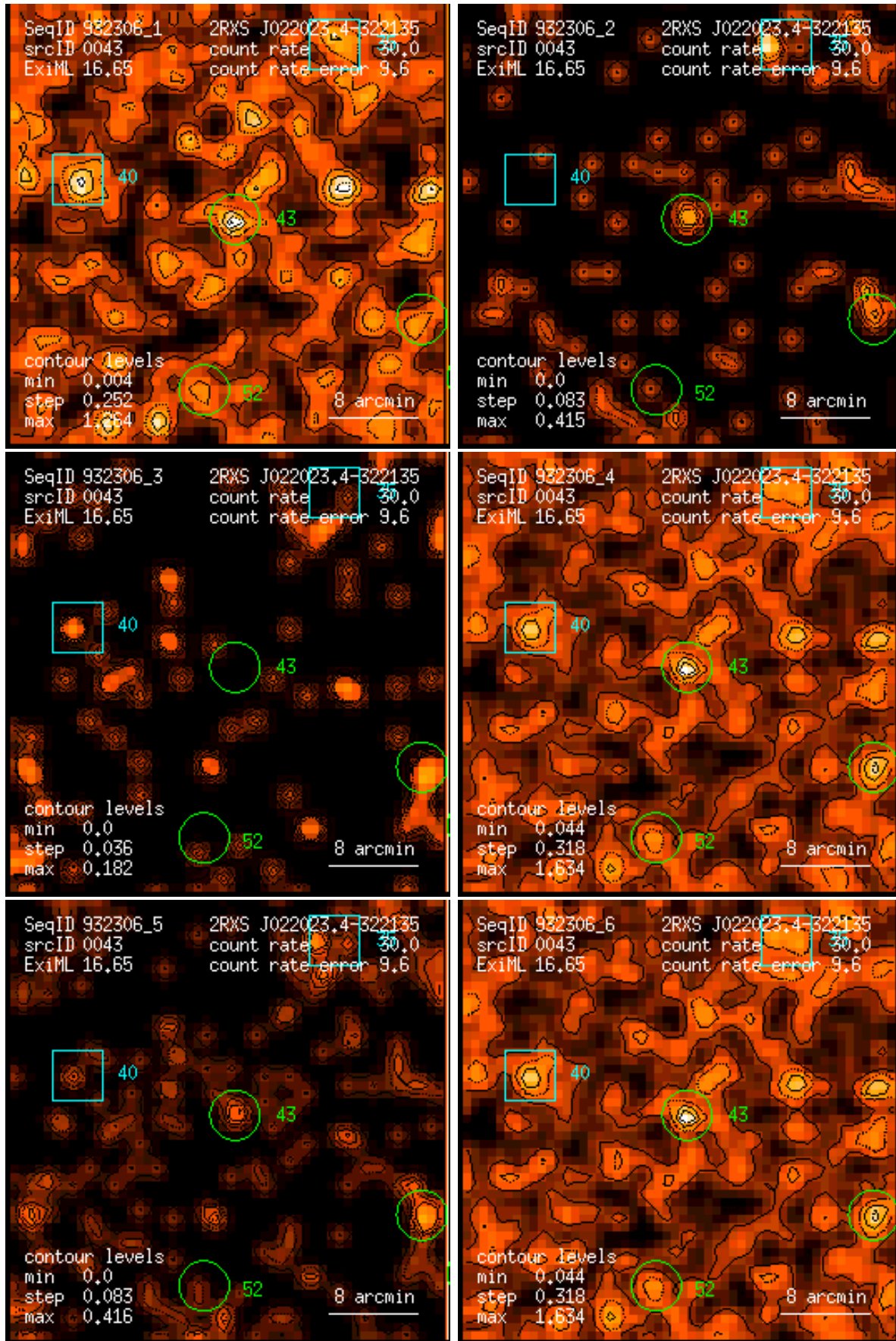
Figure 43: RASS 932306: detection 0043: band rate images, Gaussian filter: (1) PSPC channels 11 – 41, (2) 52 – 90, (3) 91 – 201, (4) 11 – 235, (5) 52 – 201, (6) 11 – 201. Broad band rates in counts/ks. Band rate contour levels in counts/ks/arcmin 2 .
