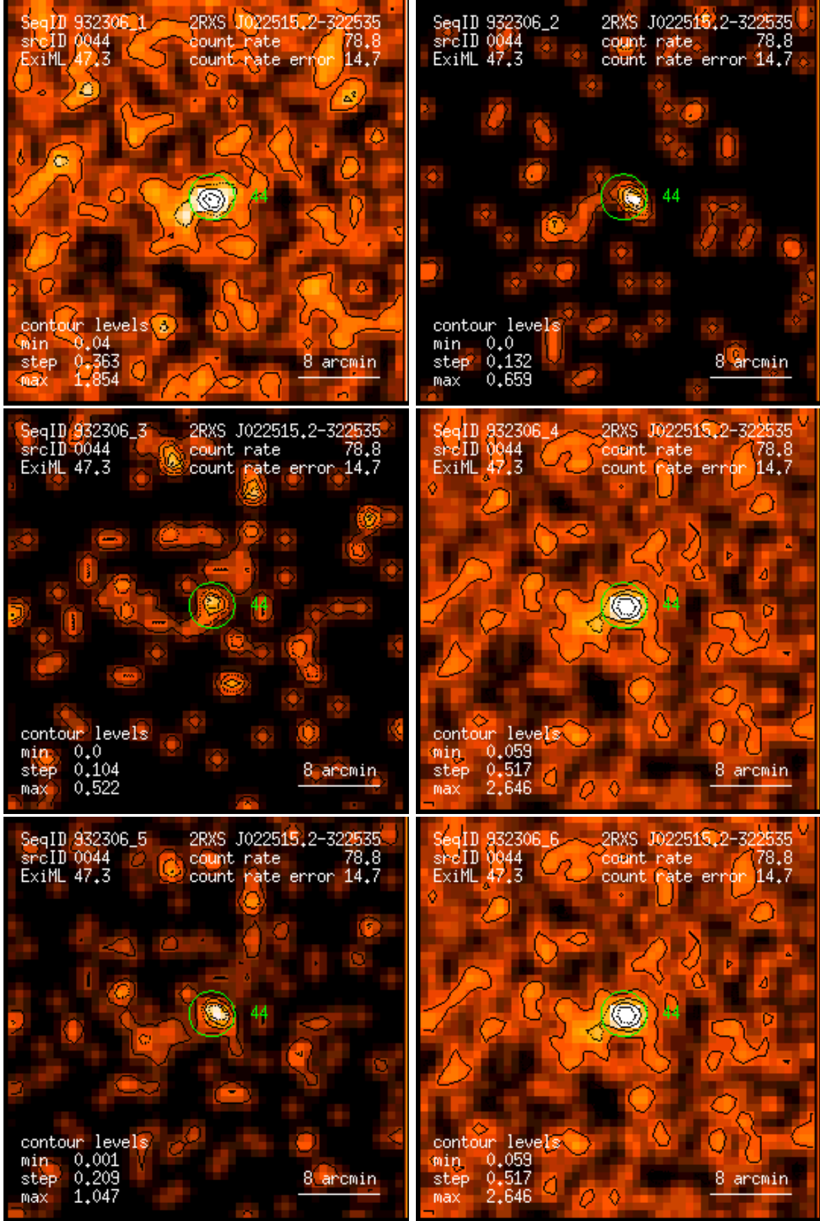
Figure 44: RASS 932306: detection 0044: band rate images, Gaussian filter: (1) PSPC channels 11 – 41, (2) 52 – 90, (3) 91 – 201, (4) 11 – 235, (5) 52 – 201, (6) 11 – 201. Broad band rates in counts/ks. Band rate contour levels in counts/ks/arcmin 2 .
