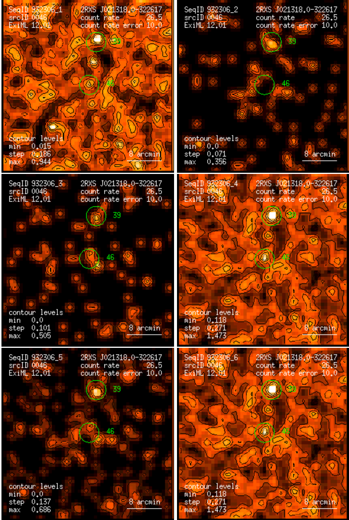
Figure 46: RASS 932306: detection 0046: band rate images, Gaussian filter: (1) PSPC channels 11 – 41, (2) 52 – 90, (3) 91 – 201, (4) 11 – 235, (5) 52 – 201, (6) 11 – 201. Broad band rates in counts/ks. Band rate contour levels in counts/ks/arcmin 2 .
