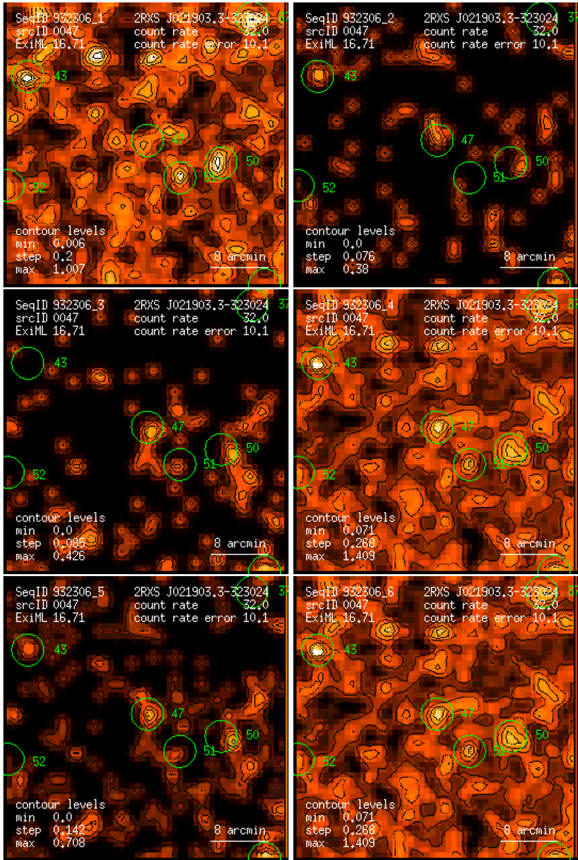
Figure 47: RASS 932306: detection 0047: band rate images, Gaussian filter: (1) PSPC channels 11 – 41, (2) 52 – 90, (3) 91 – 201, (4) 11 – 235, (5) 52 – 201, (6) 11 – 201. Broad band rates in counts/ks. Band rate contour levels in counts/ks/arcmin 2 .
