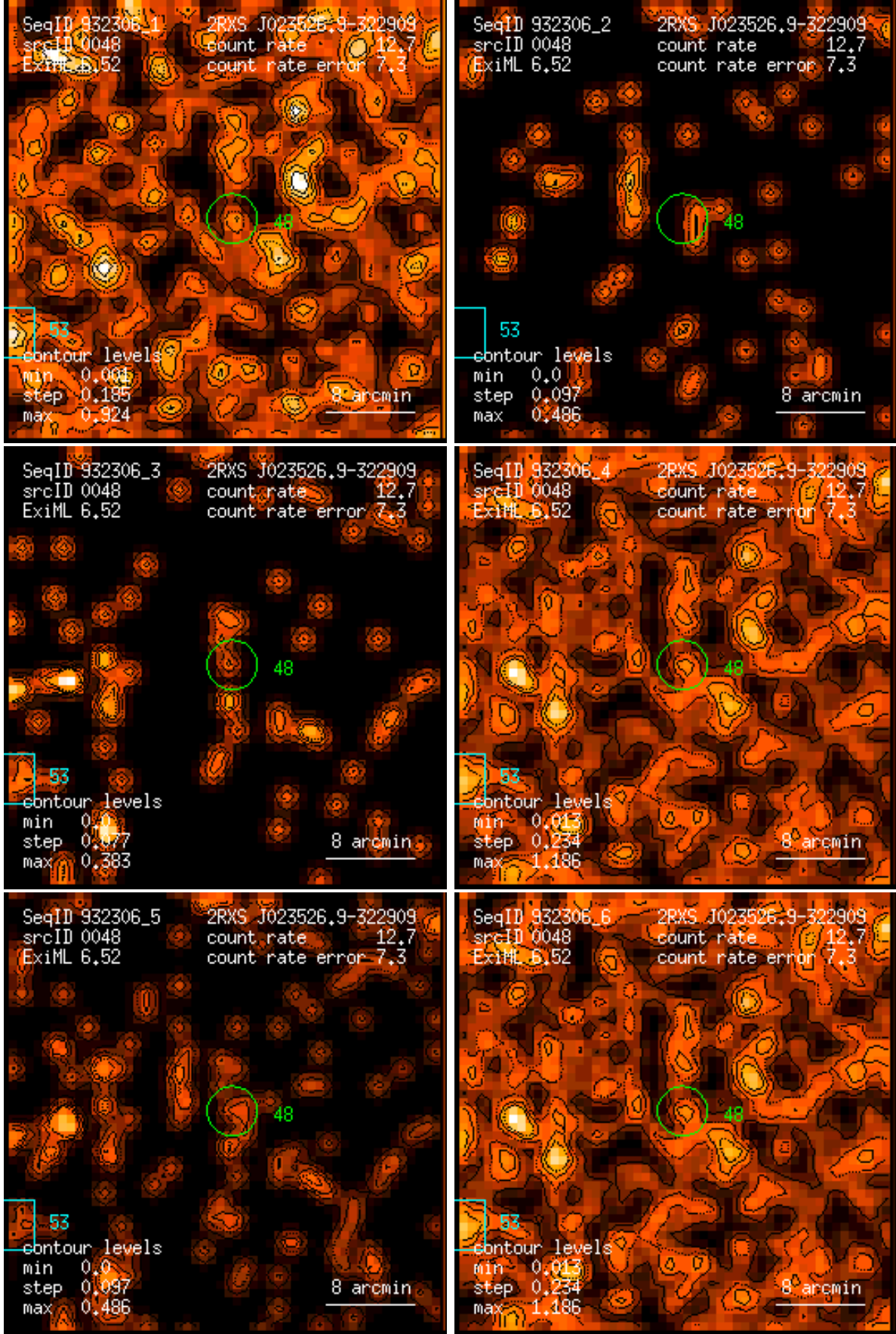
Figure 48: RASS 932306: detection 0048: band rate images, Gaussian filter: (1) PSPC channels 11 – 41, (2) 52 – 90, (3) 91 – 201, (4) 11 – 235, (5) 52 – 201, (6) 11 – 201. Broad band rates in counts/ks. Band rate contour levels in counts/ks/arcmin 2 .
