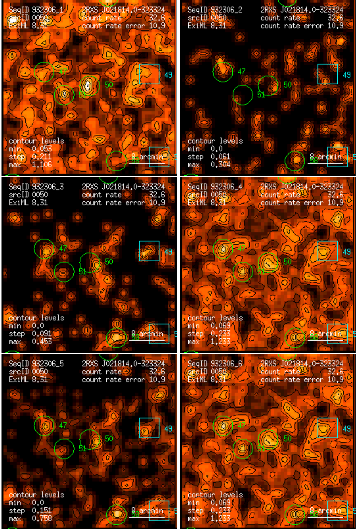
Figure 50: RASS 932306: detection 0050: band rate images, Gaussian filter: (1) PSPC channels 11 – 41, (2) 52 – 90, (3) 91 – 201, (4) 11 – 235, (5) 52 – 201, (6) 11 – 201. Broad band rates in counts/ks. Band rate contour levels in counts/ks/arcmin 2 .
