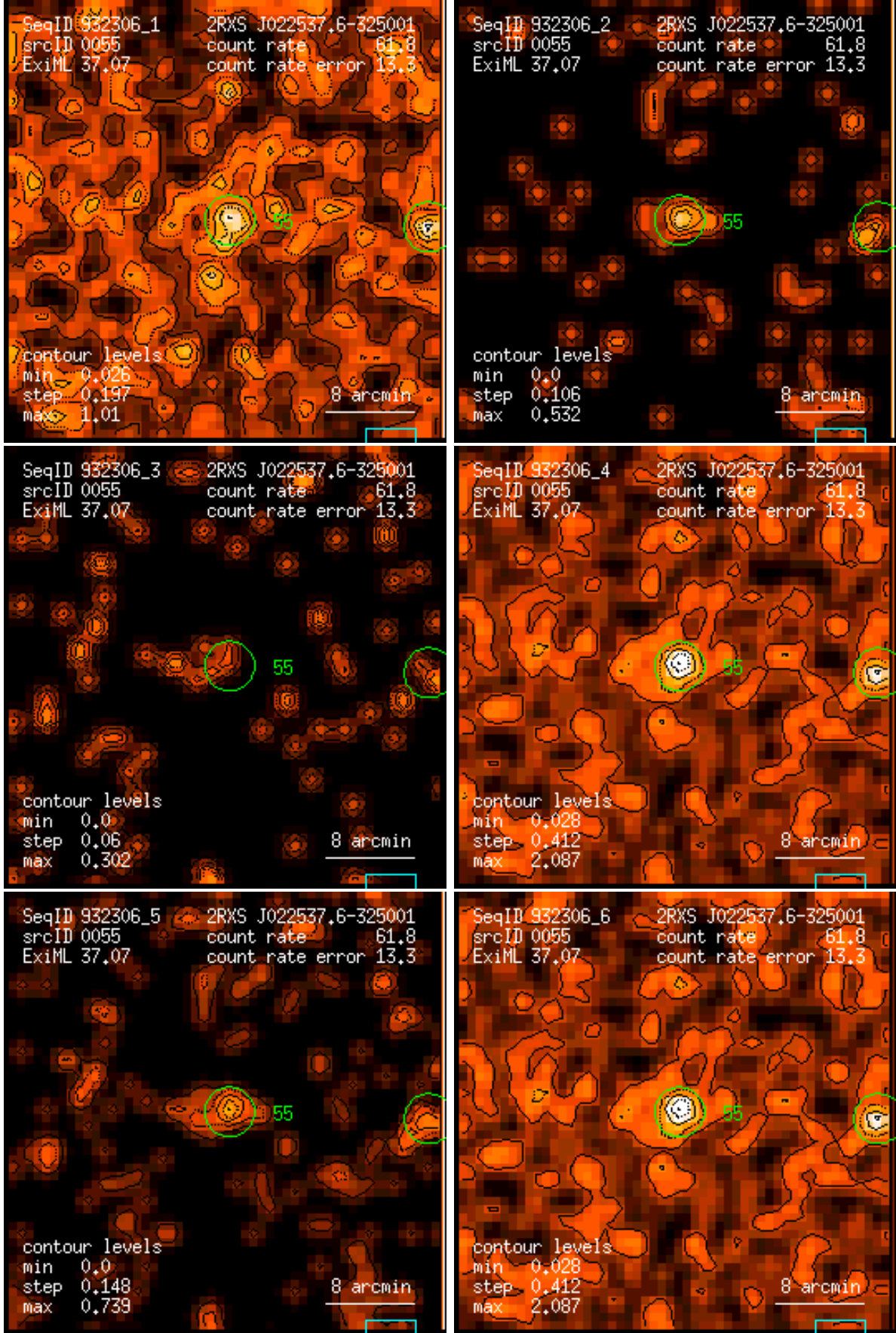
Figure 55: RASS 932306: detection 0055: band rate images, Gaussian filter: (1) PSPC channels 11 – 41, (2) 52 – 90, (3) 91 – 201, (4) 11 – 235, (5) 52 – 201, (6) 11 – 201. Broad band rates in counts/ks. Band rate contour levels in counts/ks/arcmin 2 .
