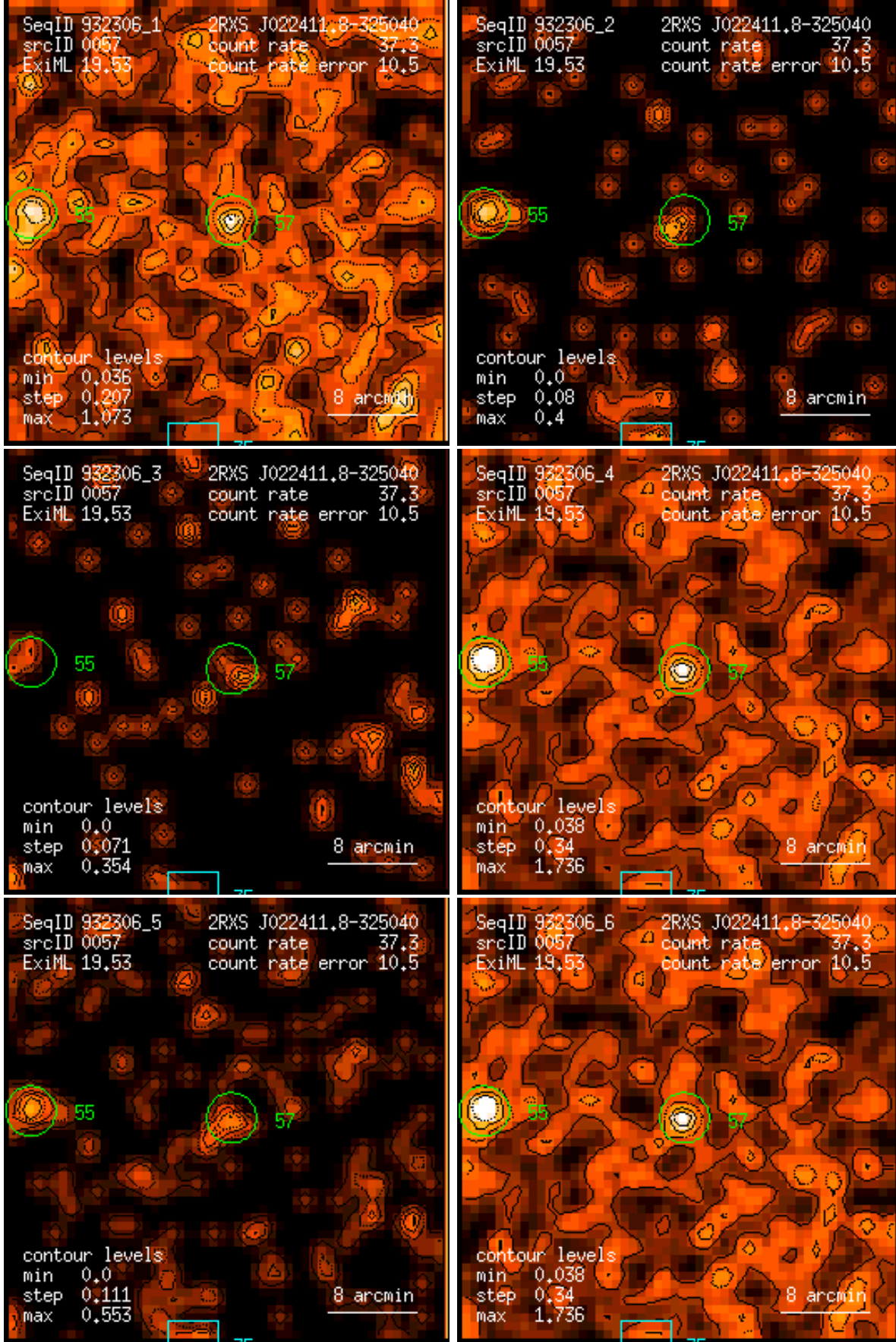
Figure 57: RASS 932306: detection 0057: band rate images, Gaussian filter: (1) PSPC channels 11 – 41, (2) 52 – 90, (3) 91 – 201, (4) 11 – 235, (5) 52 – 201, (6) 11 – 201. Broad band rates in counts/ks. Band rate contour levels in counts/ks/arcmin 2 .
