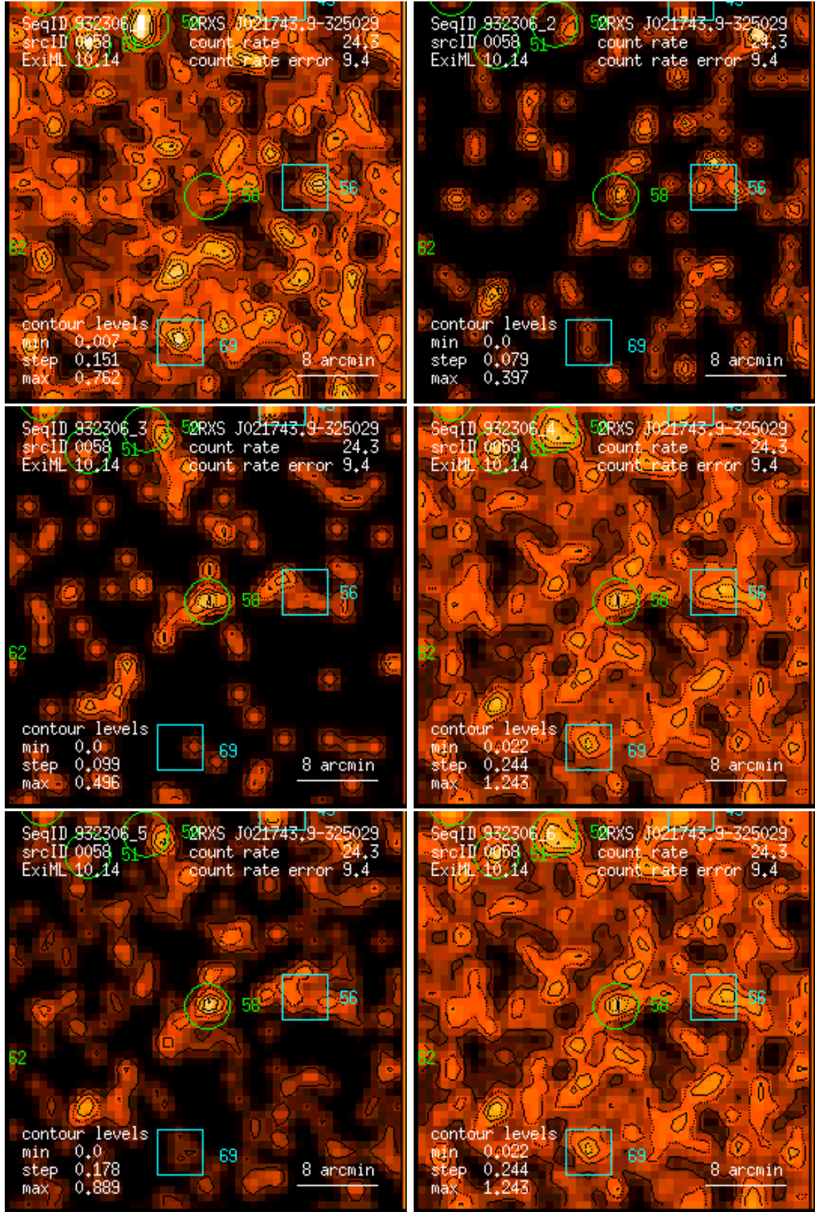
Figure 58: RASS 932306: detection 0058: band rate images, Gaussian filter: (1) PSPC channels 11 – 41, (2) 52 – 90, (3) 91 – 201, (4) 11 – 235, (5) 52 – 201, (6) 11 – 201. Broad band rates in counts/ks. Band rate contour levels in counts/ks/arcmin 2 .
