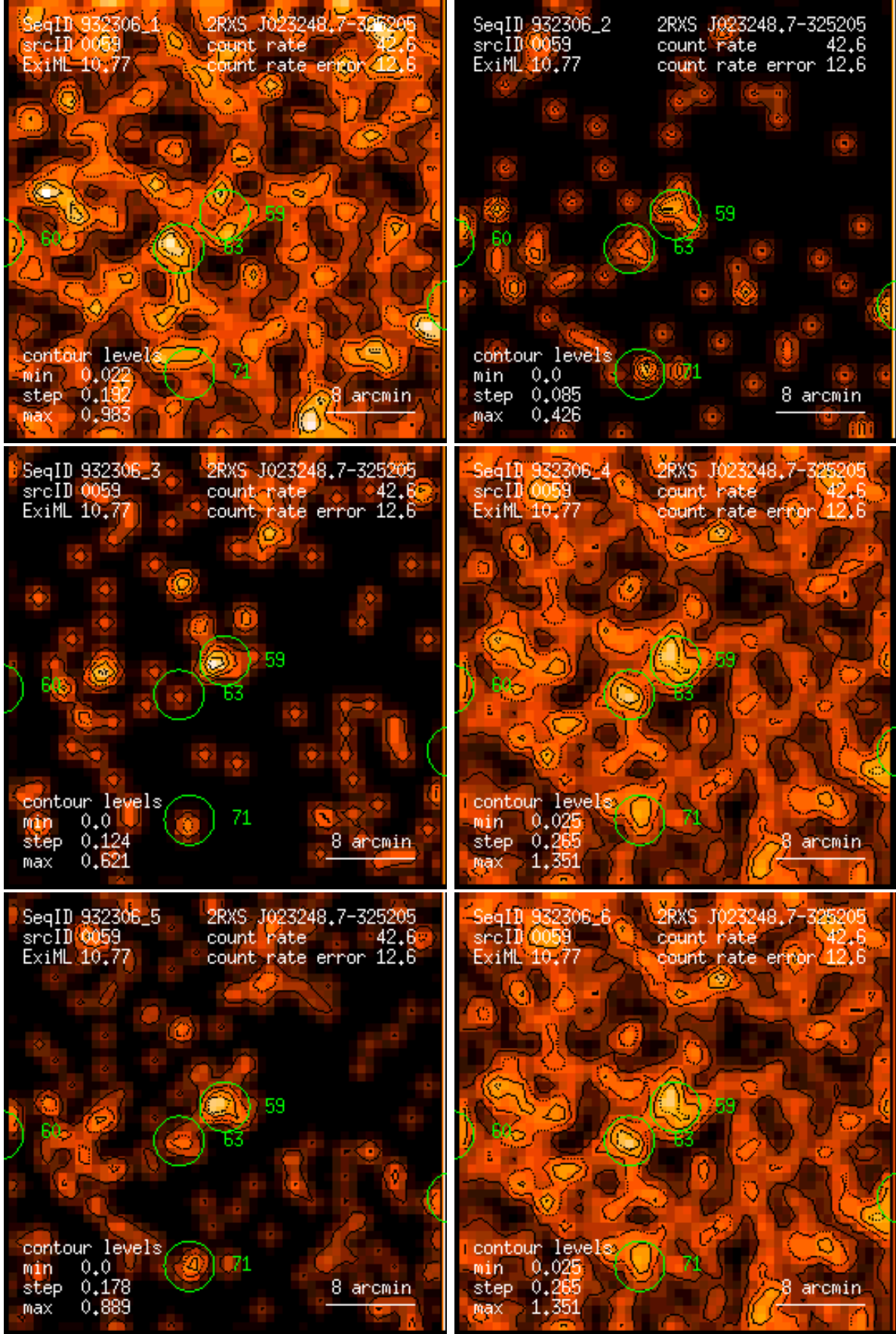
Figure 59: RASS 932306: detection 0059: band rate images, Gaussian filter: (1) PSPC channels 11 – 41, (2) 52 – 90, (3) 91 – 201, (4) 11 – 235, (5) 52 – 201, (6) 11 – 201. Broad band rates in counts/ks. Band rate contour levels in counts/ks/arcmin 2 .
