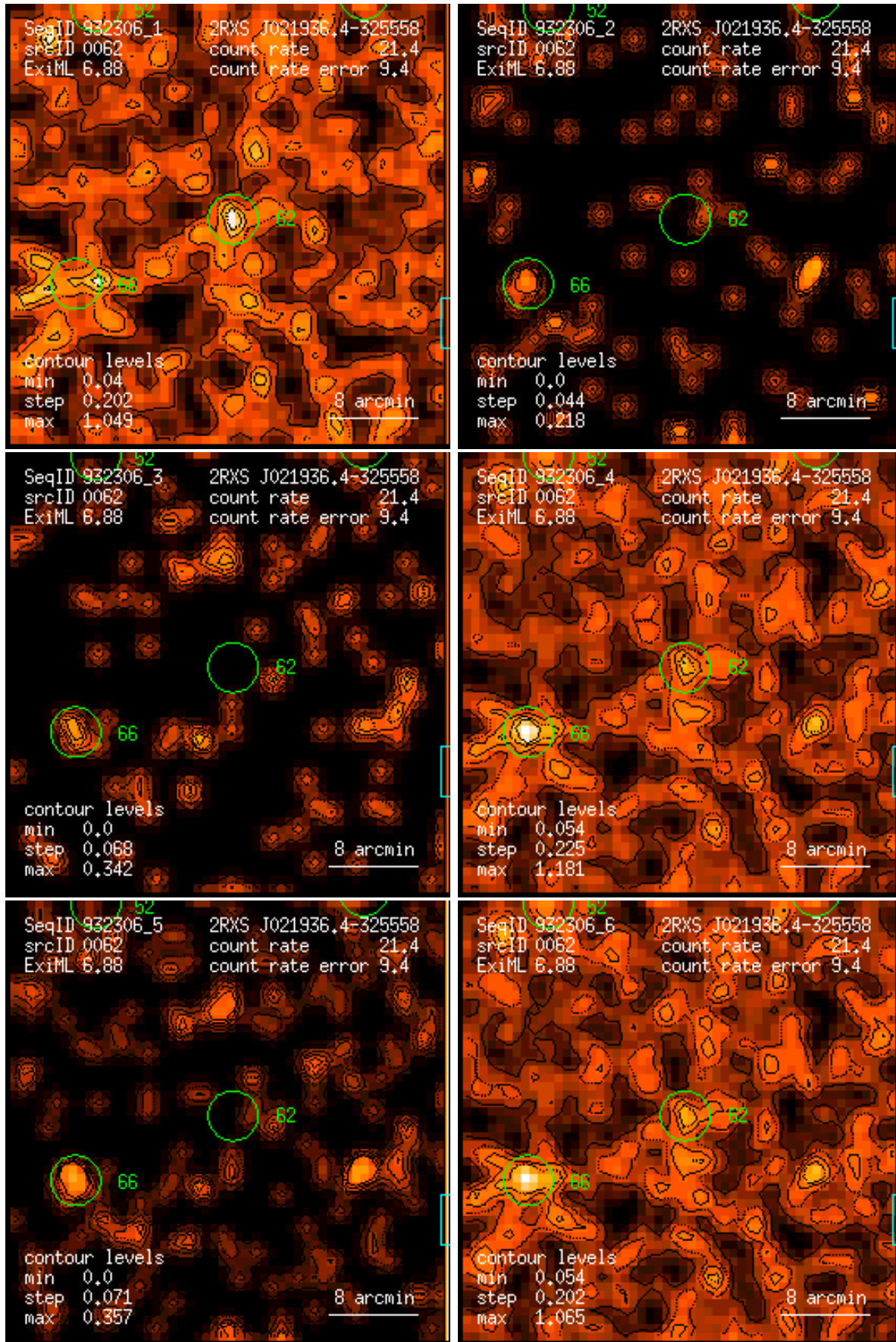
Figure 62: RASS 932306: detection 0062: band rate images, Gaussian filter: (1) PSPC channels 11 – 41, (2) 52 – 90, (3) 91 – 201, (4) 11 – 235, (5) 52 – 201, (6) 11 – 201. Broad band rates in counts/ks. Band rate contour levels in counts/ks/arcmin 2 .
