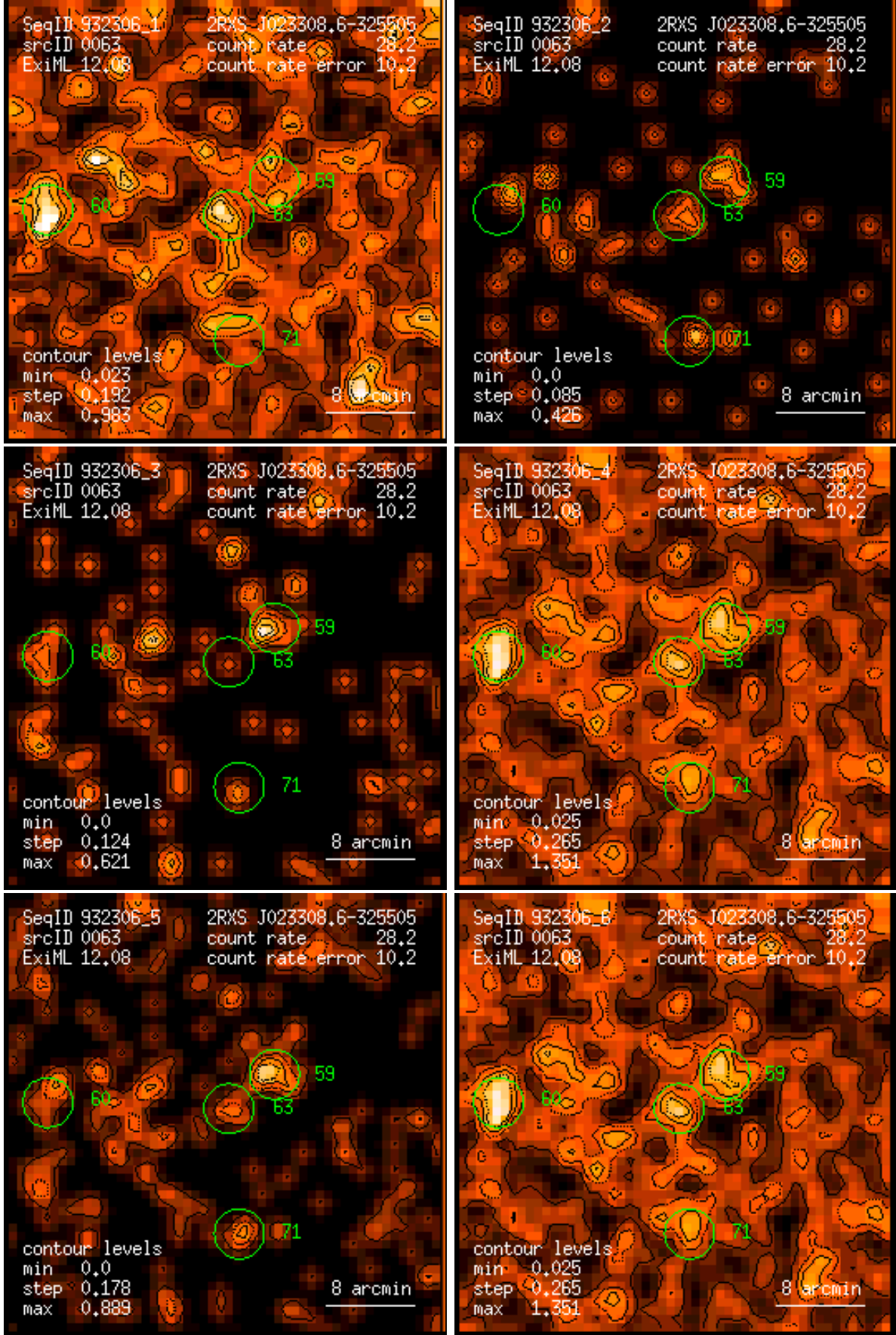
Figure 63: RASS 932306: detection 0063: band rate images, Gaussian filter: (1) PSPC channels 11 – 41, (2) 52 – 90, (3) 91 – 201, (4) 11 – 235, (5) 52 – 201, (6) 11 – 201. Broad band rates in counts/ks. Band rate contour levels in counts/ks/arcmin 2 .
