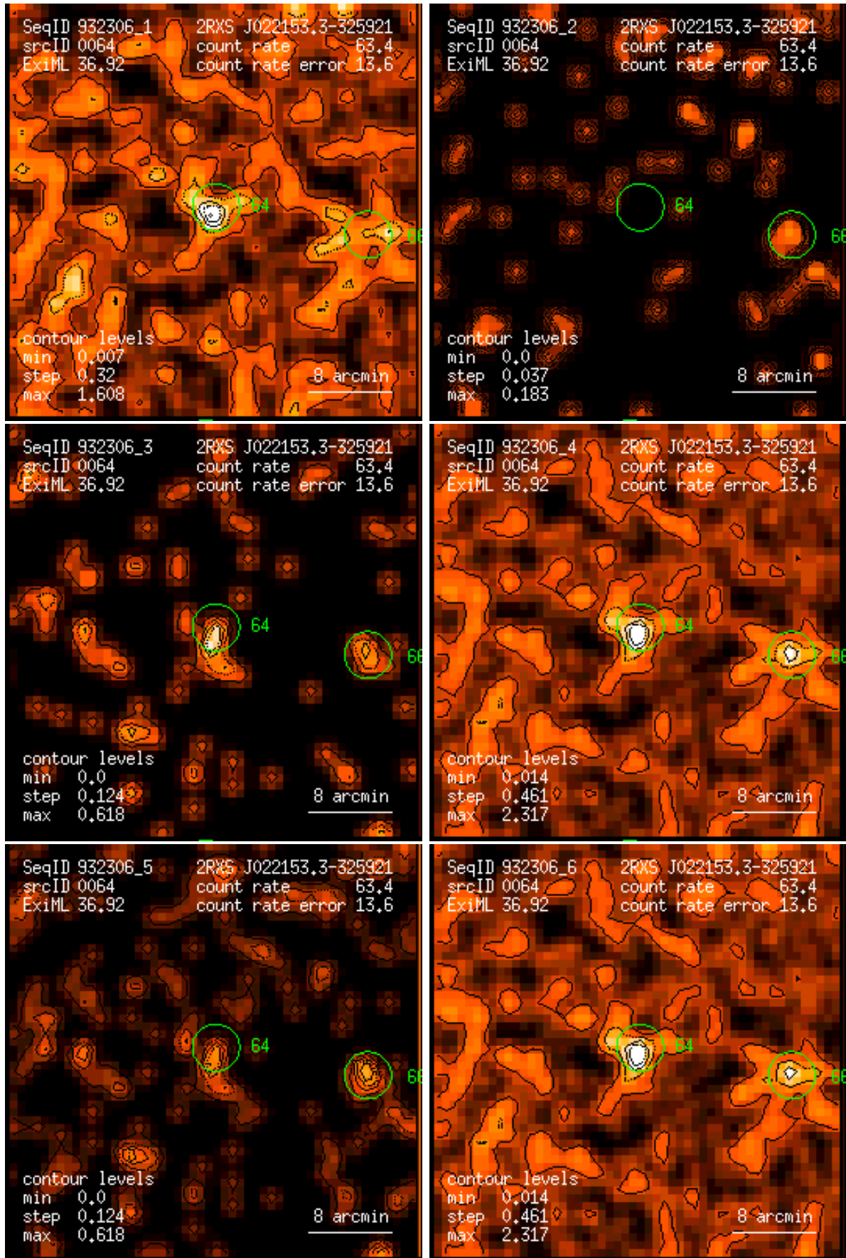
Figure 64: RASS 932306: detection 0064: band rate images, Gaussian filter: (1) PSPC channels 11 – 41, (2) 52 – 90, (3) 91 – 201, (4) 11 – 235, (5) 52 – 201, (6) 11 – 201. Broad band rates in counts/ks. Band rate contour levels in counts/ks/arcmin 2 .
