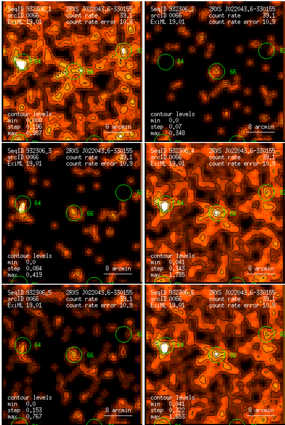
Figure 66: RASS 932306: detection 0066: band rate images, Gaussian filter: (1) PSPC channels 11 – 41, (2) 52 – 90, (3) 91 – 201, (4) 11 – 235, (5) 52 – 201, (6) 11 – 201. Broad band rates in counts/ks. Band rate contour levels in counts/ks/arcmin 2 .
