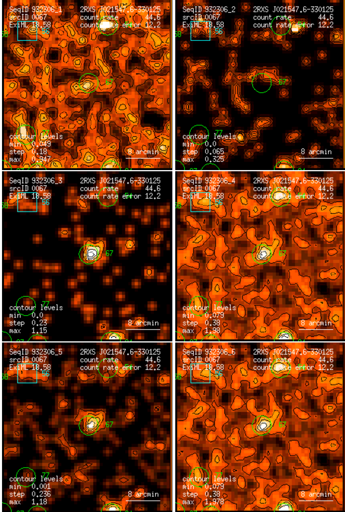
Figure 67: RASS 932306: detection 0067: band rate images, Gaussian filter: (1) PSPC channels 11 – 41, (2) 52 – 90, (3) 91 – 201, (4) 11 – 235, (5) 52 – 201, (6) 11 – 201. Broad band rates in counts/ks. Band rate contour levels in counts/ks/arcmin 2 .
