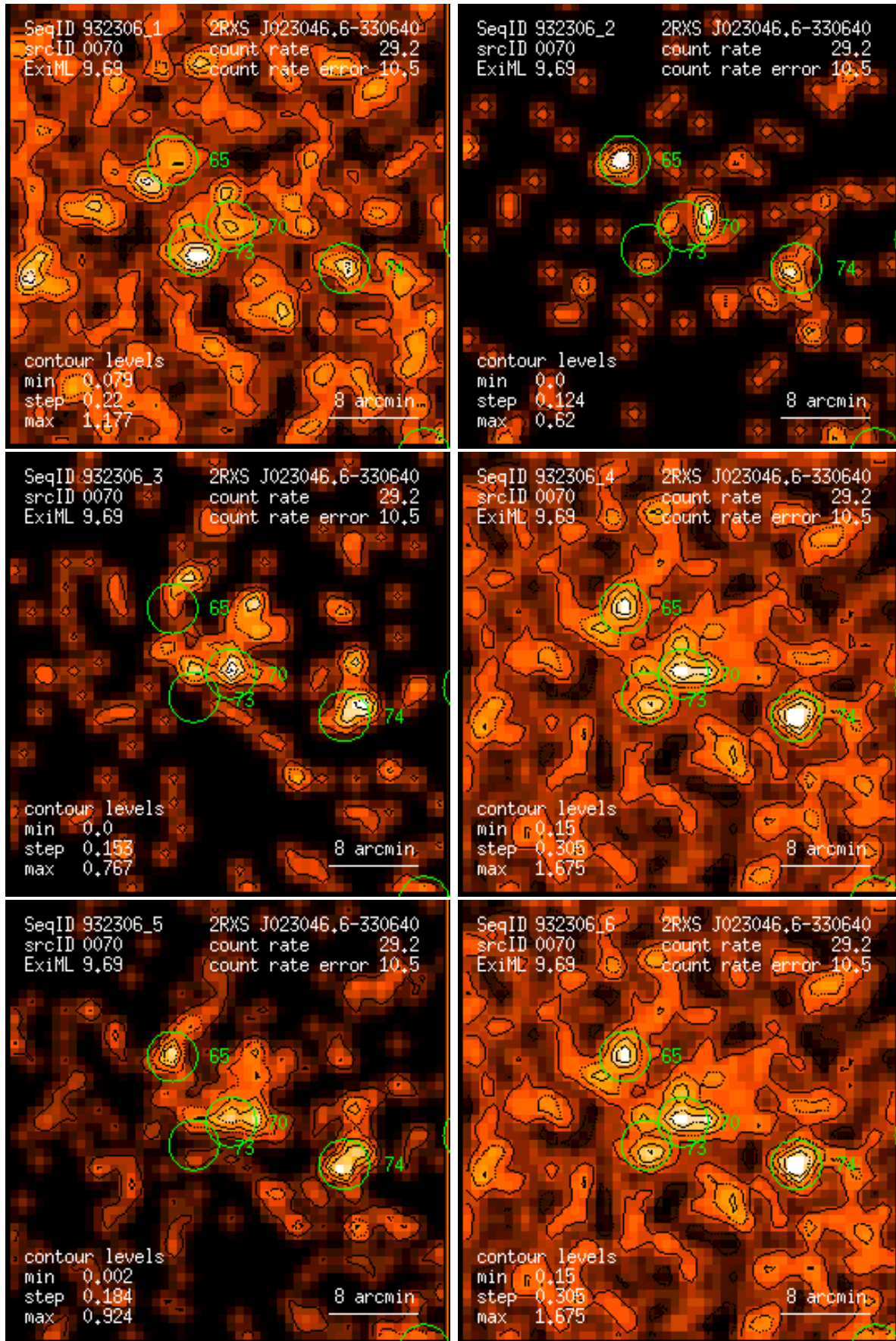
Figure 70: RASS 932306: detection 0070: band rate images, Gaussian filter: (1) PSPC channels 11 – 41, (2) 52 – 90, (3) 91 – 201, (4) 11 – 235, (5) 52 – 201, (6) 11 – 201. Broad band rates in counts/ks. Band rate contour levels in counts/ks/arcmin 2 .
