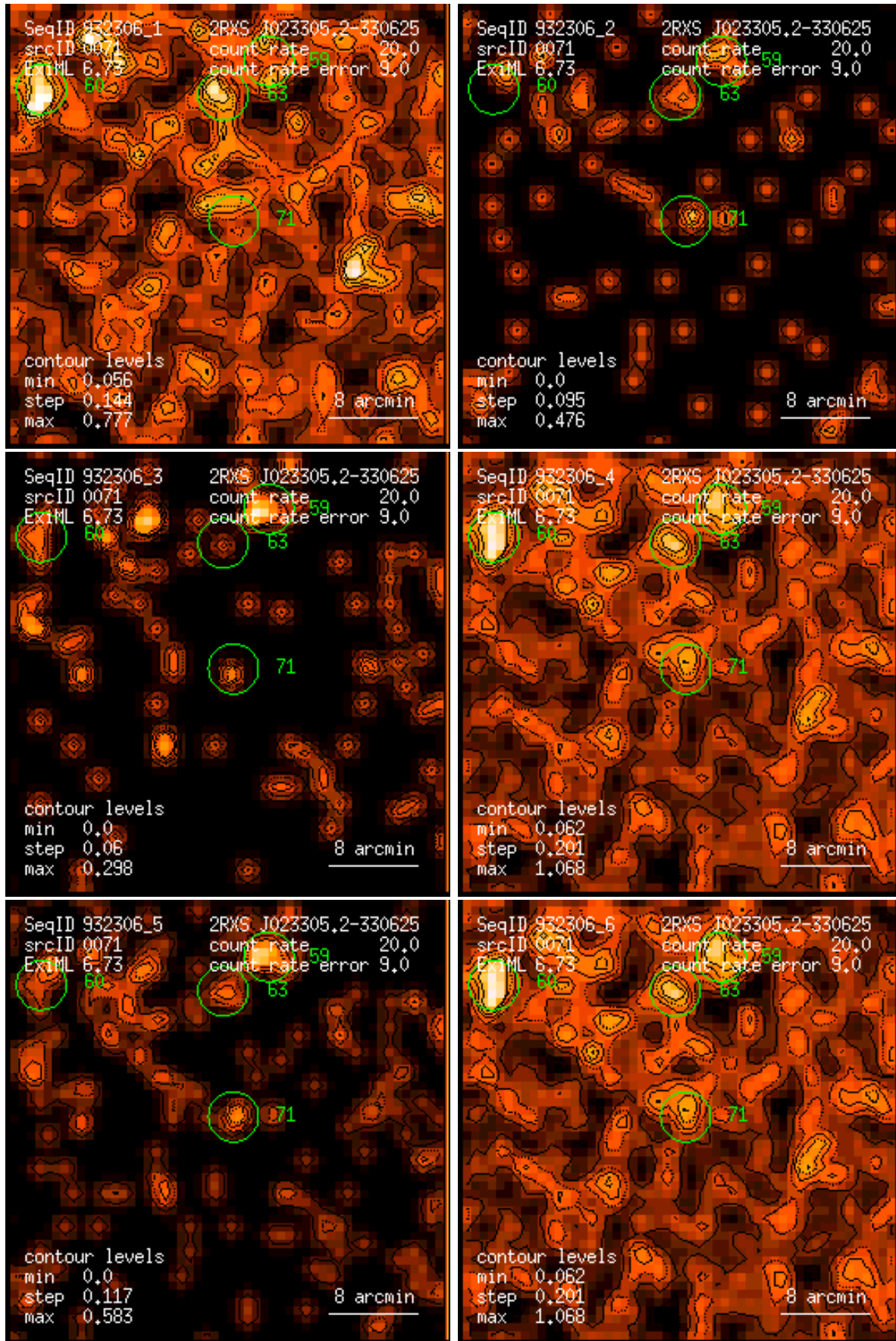
Figure 71: RASS 932306: detection 0071: band rate images, Gaussian filter: (1) PSPC channels 11 – 41, (2) 52 – 90, (3) 91 – 201, (4) 11 – 235, (5) 52 – 201, (6) 11 – 201. Broad band rates in counts/ks. Band rate contour levels in counts/ks/arcmin 2 .
