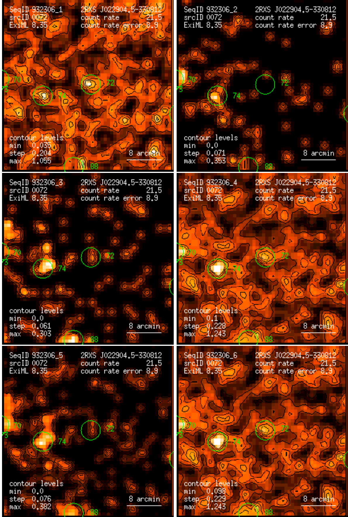
Figure 72: RASS 932306: detection 0072: band rate images, Gaussian filter: (1) PSPC channels 11 – 41, (2) 52 – 90, (3) 91 – 201, (4) 11 – 235, (5) 52 – 201, (6) 11 – 201. Broad band rates in counts/ks. Band rate contour levels in counts/ks/arcmin 2 .
