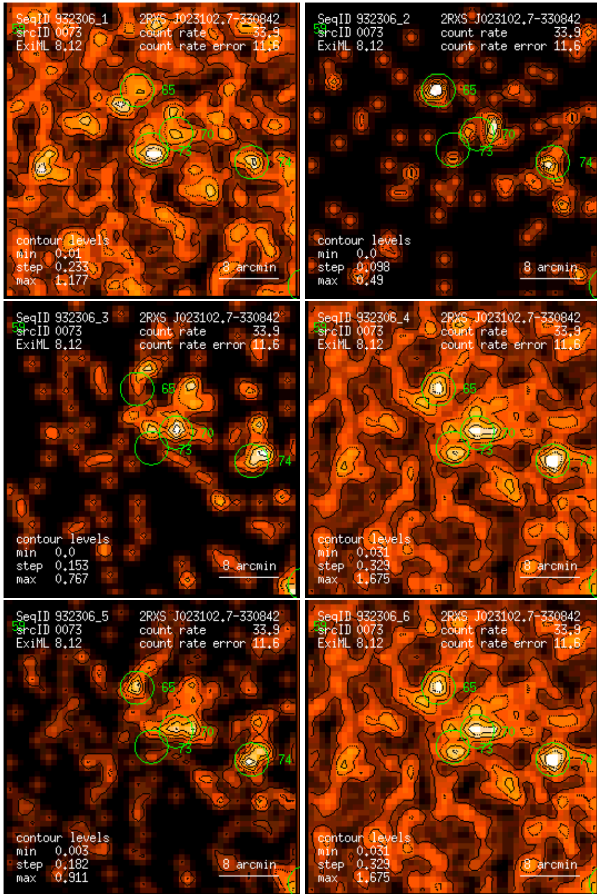
Figure 73: RASS 932306: detection 0073: band rate images, Gaussian filter: (1) PSPC channels 11 – 41, (2) 52 – 90, (3) 91 – 201, (4) 11 – 235, (5) 52 – 201, (6) 11 – 201. Broad band rates in counts/ks. Band rate contour levels in counts/ks/arcmin 2 .
