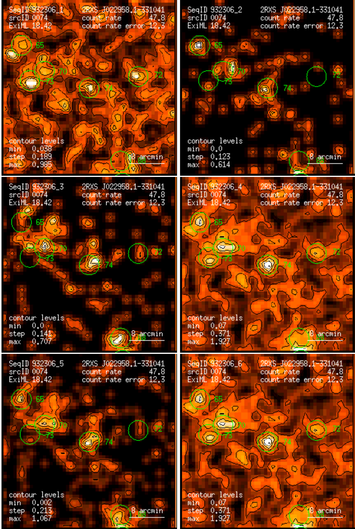
Figure 74: RASS 932306: detection 0074: band rate images, Gaussian filter: (1) PSPC channels 11 – 41, (2) 52 – 90, (3) 91 – 201, (4) 11 – 235, (5) 52 – 201, (6) 11 – 201. Broad band rates in counts/ks. Band rate contour levels in counts/ks/arcmin 2 .
