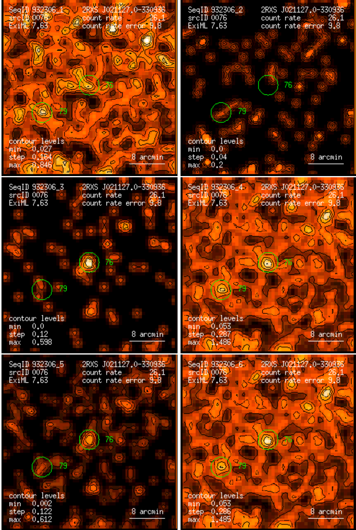
Figure 76: RASS 932306: detection 0076: band rate images, Gaussian filter: (1) PSPC channels 11 – 41, (2) 52 – 90, (3) 91 – 201, (4) 11 – 235, (5) 52 – 201, (6) 11 – 201. Broad band rates in counts/ks. Band rate contour levels in counts/ks/arcmin 2 .
