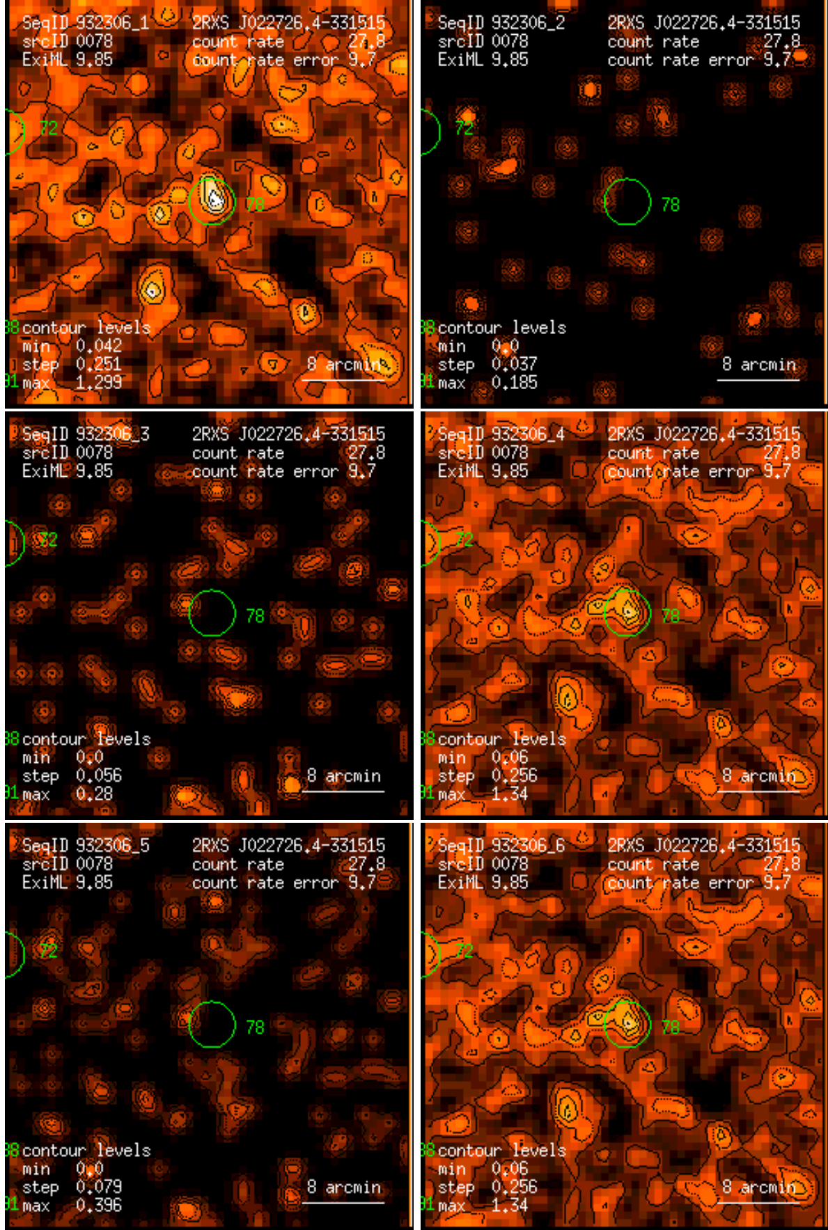
Figure 78: RASS 932306: detection 0078: band rate images, Gaussian filter: (1) PSPC channels 11 – 41, (2) 52 – 90, (3) 91 – 201, (4) 11 – 235, (5) 52 – 201, (6) 11 – 201. Broad band rates in counts/ks. Band rate contour levels in counts/ks/arcmin 2 .
