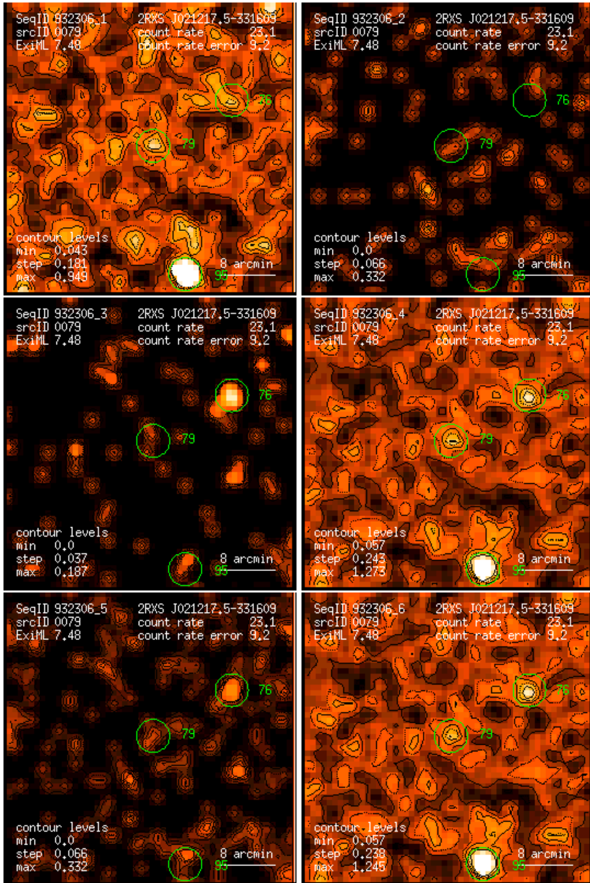
Figure 79: RASS 932306: detection 0079: band rate images, Gaussian filter: (1) PSPC channels 11 – 41, (2) 52 – 90, (3) 91 – 201, (4) 11 – 235, (5) 52 – 201, (6) 11 – 201. Broad band rates in counts/ks. Band rate contour levels in counts/ks/arcmin 2 .
