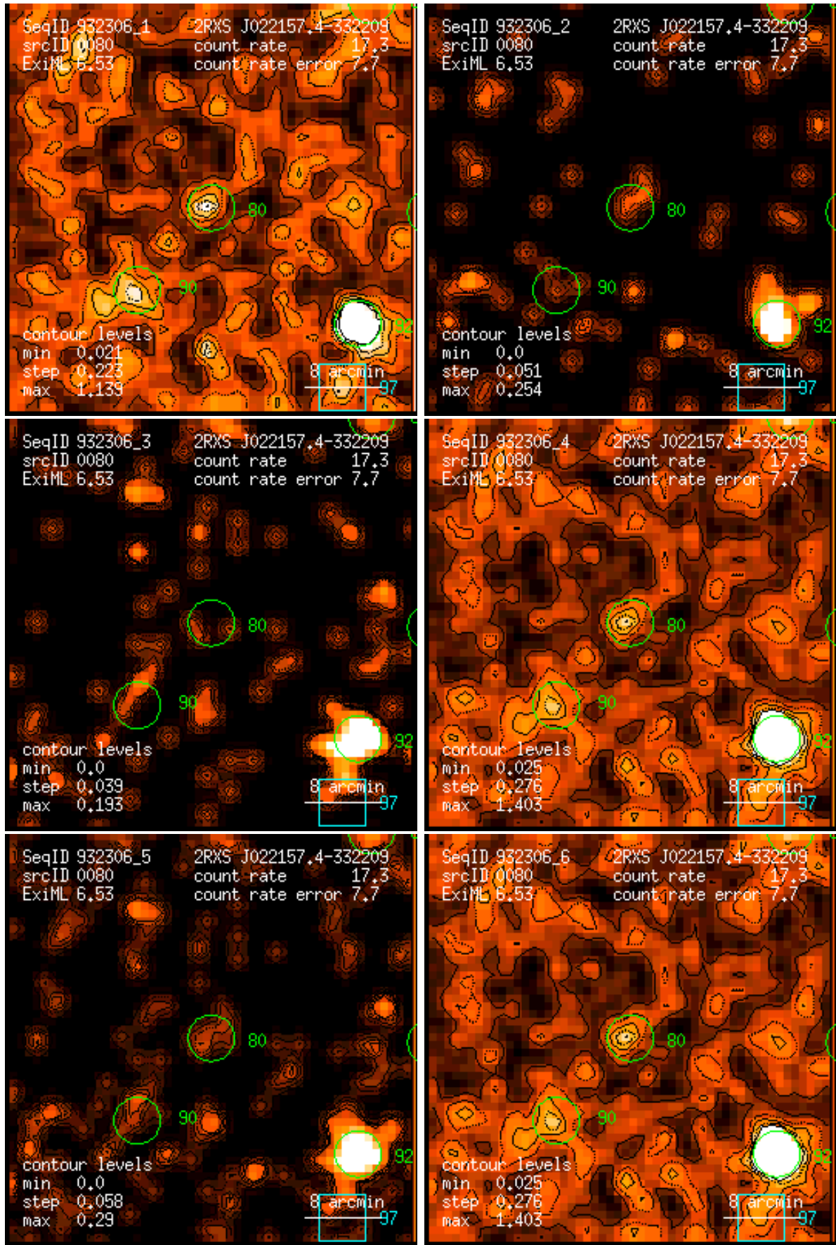
Figure 80: RASS 932306: detection 0080: band rate images, Gaussian filter: (1) PSPC channels 11 – 41, (2) 52 – 90, (3) 91 – 201, (4) 11 – 235, (5) 52 – 201, (6) 11 – 201. Broad band rates in counts/ks. Band rate contour levels in counts/ks/arcmin 2 .
