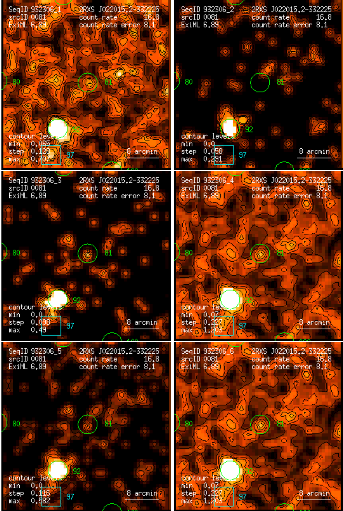
Figure 81: RASS 932306: detection 0081: band rate images, Gaussian filter: (1) PSPC channels 11 – 41, (2) 52 – 90, (3) 91 – 201, (4) 11 – 235, (5) 52 – 201, (6) 11 – 201. Broad band rates in counts/ks. Band rate contour levels in counts/ks/arcmin 2 .
