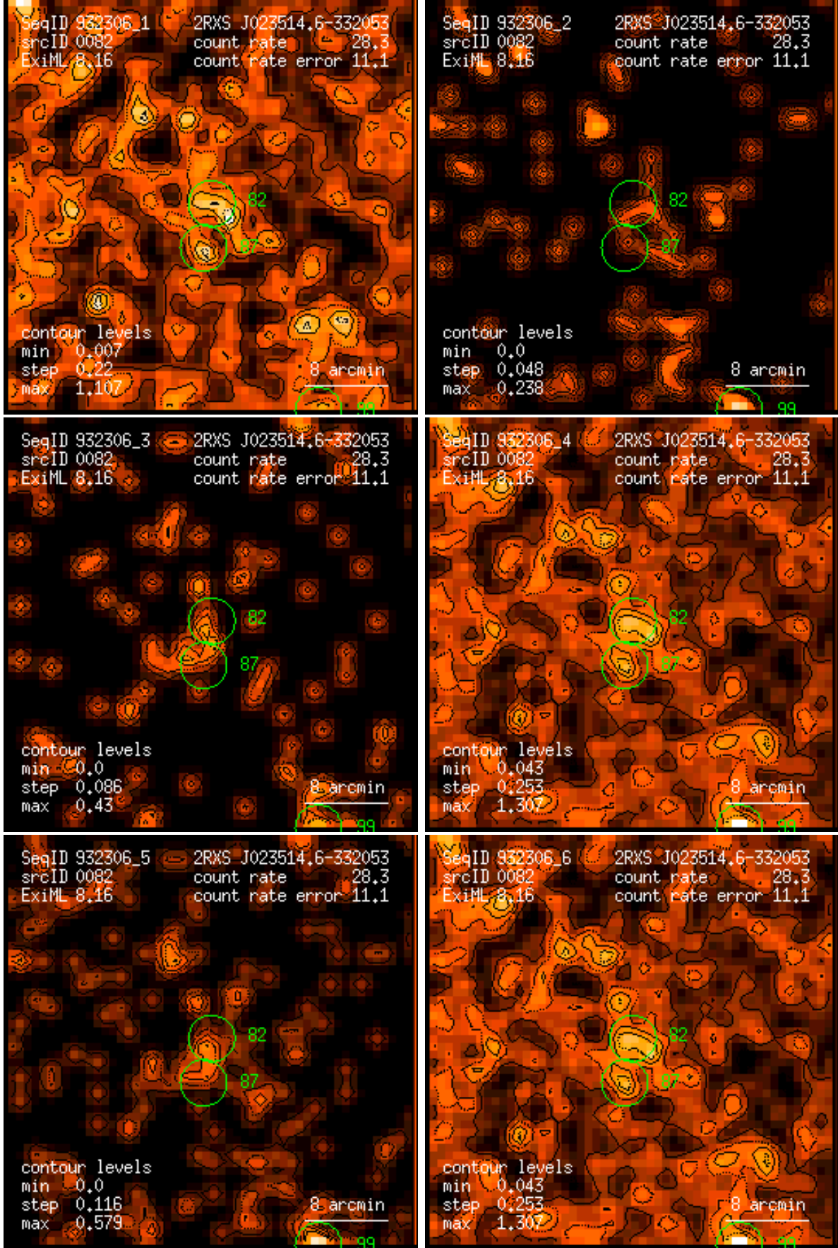
Figure 82: RASS 932306: detection 0082: band rate images, Gaussian filter: (1) PSPC channels 11 – 41, (2) 52 – 90, (3) 91 – 201, (4) 11 – 235, (5) 52 – 201, (6) 11 – 201. Broad band rates in counts/ks. Band rate contour levels in counts/ks/arcmin 2 .
