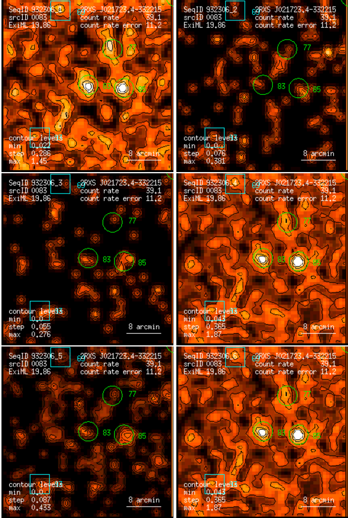
Figure 83: RASS 932306: detection 0083: band rate images, Gaussian filter: (1) PSPC channels 11 – 41, (2) 52 – 90, (3) 91 – 201, (4) 11 – 235, (5) 52 – 201, (6) 11 – 201. Broad band rates in counts/ks. Band rate contour levels in counts/ks/arcmin 2 .
