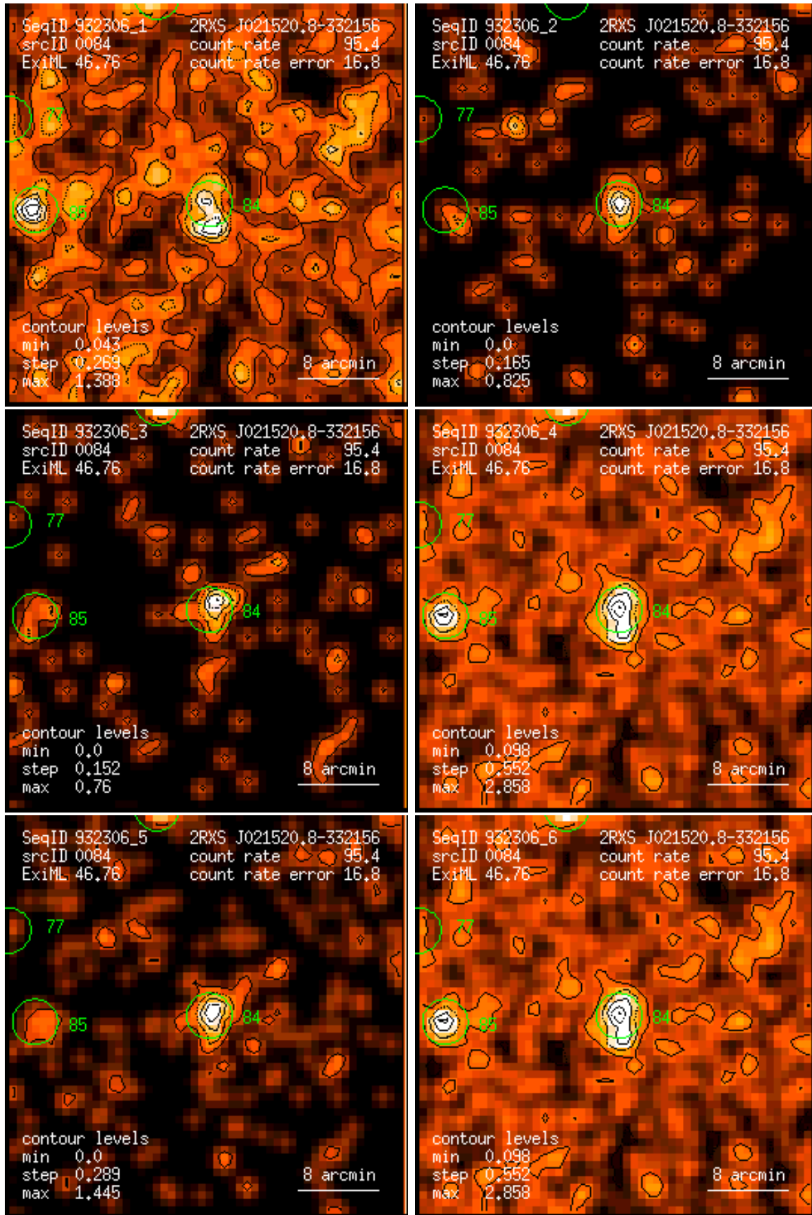
Figure 84: RASS 932306: detection 0084: band rate images, Gaussian filter: (1) PSPC channels 11 – 41, (2) 52 – 90, (3) 91 – 201, (4) 11 – 235, (5) 52 – 201, (6) 11 – 201. Broad band rates in counts/ks. Band rate contour levels in counts/ks/arcmin 2 .
