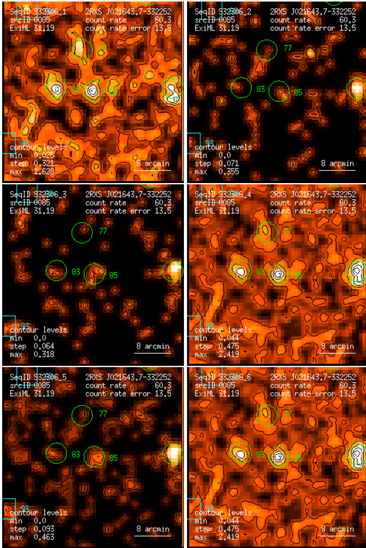
Figure 85: RASS 932306: detection 0085: band rate images, Gaussian filter: (1) PSPC channels 11 – 41, (2) 52 – 90, (3) 91 – 201, (4) 11 – 235, (5) 52 – 201, (6) 11 – 201. Broad band rates in counts/ks. Band rate contour levels in counts/ks/arcmin 2 .
