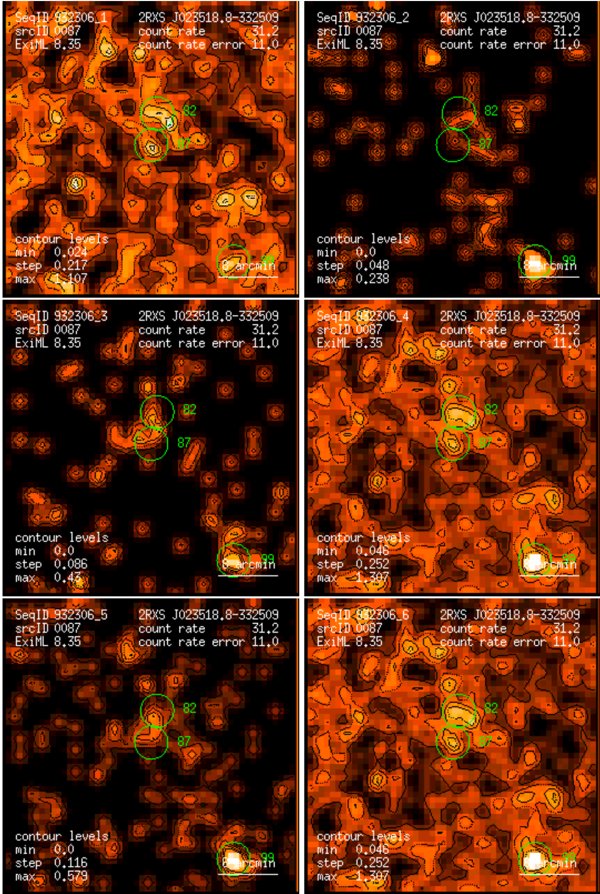
Figure 87: RASS 932306: detection 0087: band rate images, Gaussian filter: (1) PSPC channels 11 – 41, (2) 52 – 90, (3) 91 – 201, (4) 11 – 235, (5) 52 – 201, (6) 11 – 201. Broad band rates in counts/ks. Band rate contour levels in counts/ks/arcmin 2 .
