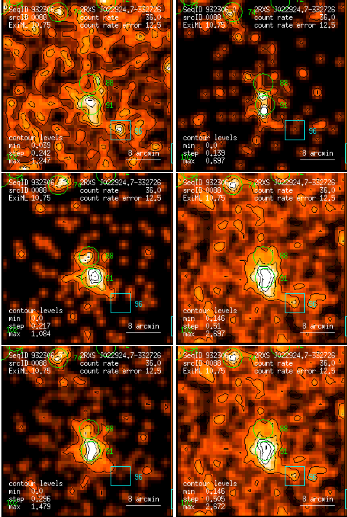
Figure 88: RASS 932306: detection 0088: band rate images, Gaussian filter: (1) PSPC channels 11 – 41, (2) 52 – 90, (3) 91 – 201, (4) 11 – 235, (5) 52 – 201, (6) 11 – 201. Broad band rates in counts/ks. Band rate contour levels in counts/ks/arcmin 2 .
