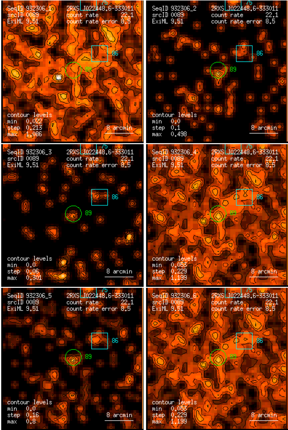
Figure 89: RASS 932306: detection 0089: band rate images, Gaussian filter: (1) PSPC channels 11 – 41, (2) 52 – 90, (3) 91 – 201, (4) 11 – 235, (5) 52 – 201, (6) 11 – 201. Broad band rates in counts/ks. Band rate contour levels in counts/ks/arcmin 2 .
