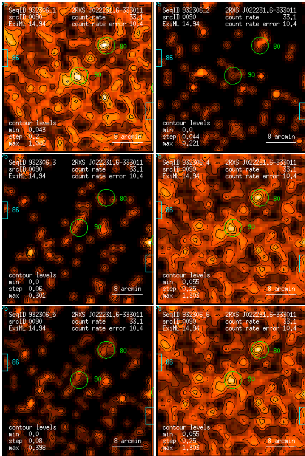
Figure 90: RASS 932306: detection 0090: band rate images, Gaussian filter: (1) PSPC channels 11 – 41, (2) 52 – 90, (3) 91 – 201, (4) 11 – 235, (5) 52 – 201, (6) 11 – 201. Broad band rates in counts/ks. Band rate contour levels in counts/ks/arcmin 2 .
