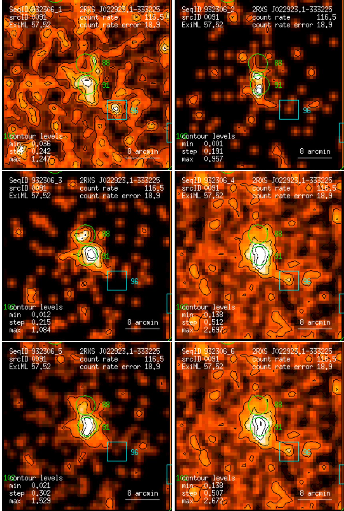
Figure 91: RASS 932306: detection 0091: band rate images, Gaussian filter: (1) PSPC channels 11 – 41, (2) 52 – 90, (3) 91 – 201, (4) 11 – 235, (5) 52 – 201, (6) 11 – 201. Broad band rates in counts/ks. Band rate contour levels in counts/ks/arcmin 2 .
