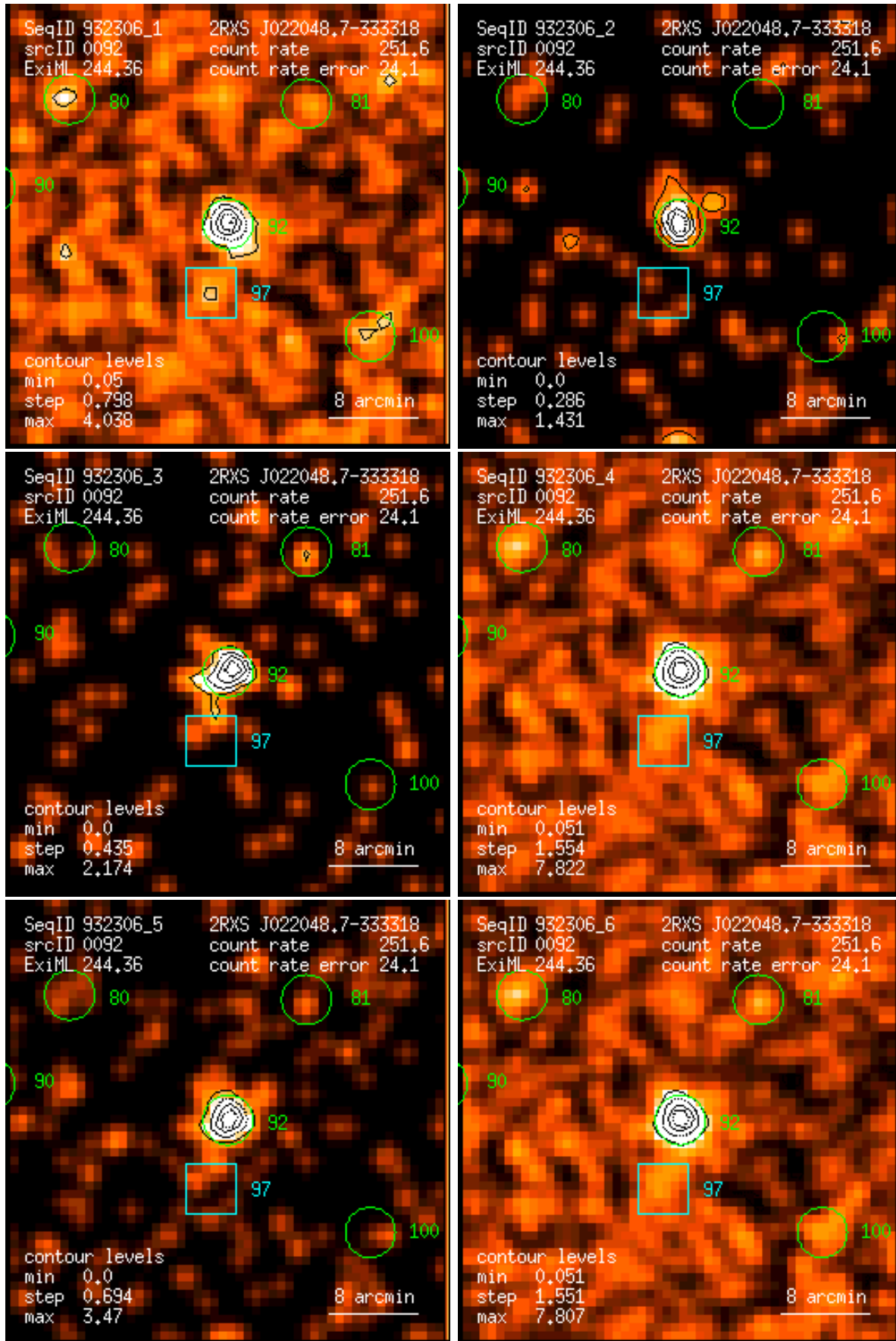
Figure 92: RASS 932306: detection 0092: band rate images, Gaussian filter: (1) PSPC channels 11 – 41, (2) 52 – 90, (3) 91 – 201, (4) 11 – 235, (5) 52 – 201, (6) 11 – 201. Broad band rates in counts/ks. Band rate contour levels in counts/ks/arcmin 2 .
